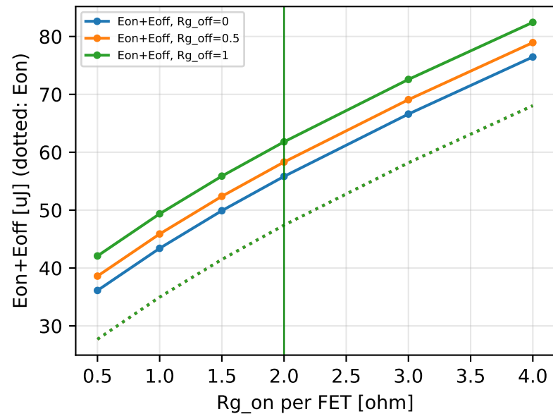
Gate-resistor study, 75 V / 160 A, 2 x EPC2361 per switch, Q3D building-block parasitics
