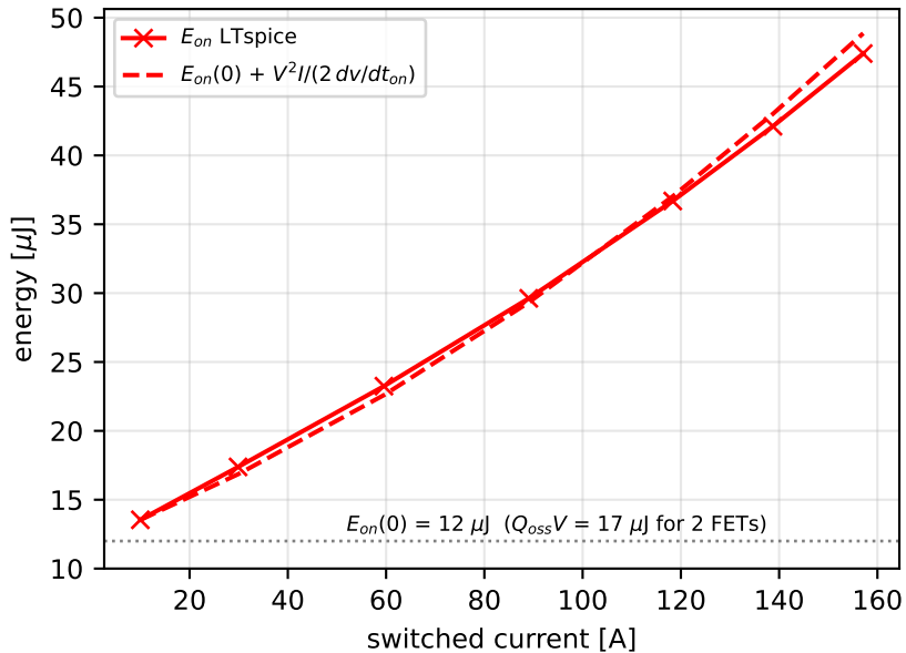
turn-on: capacitive part + dv/dt -limited overlap
