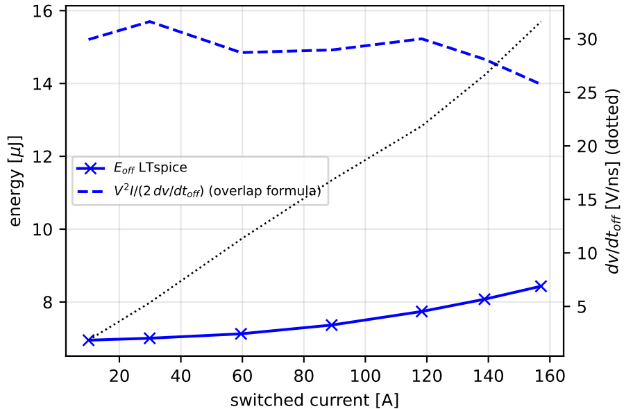
turn-off: channel closes before V_{DS} rises
