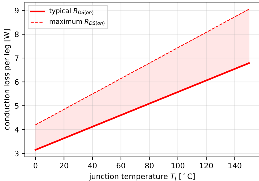
I_{rms} = 100 A, P_{cond} = I_{rms}^2 R_{DS(on)}(T_j)/2 (SPWM = SVM)
