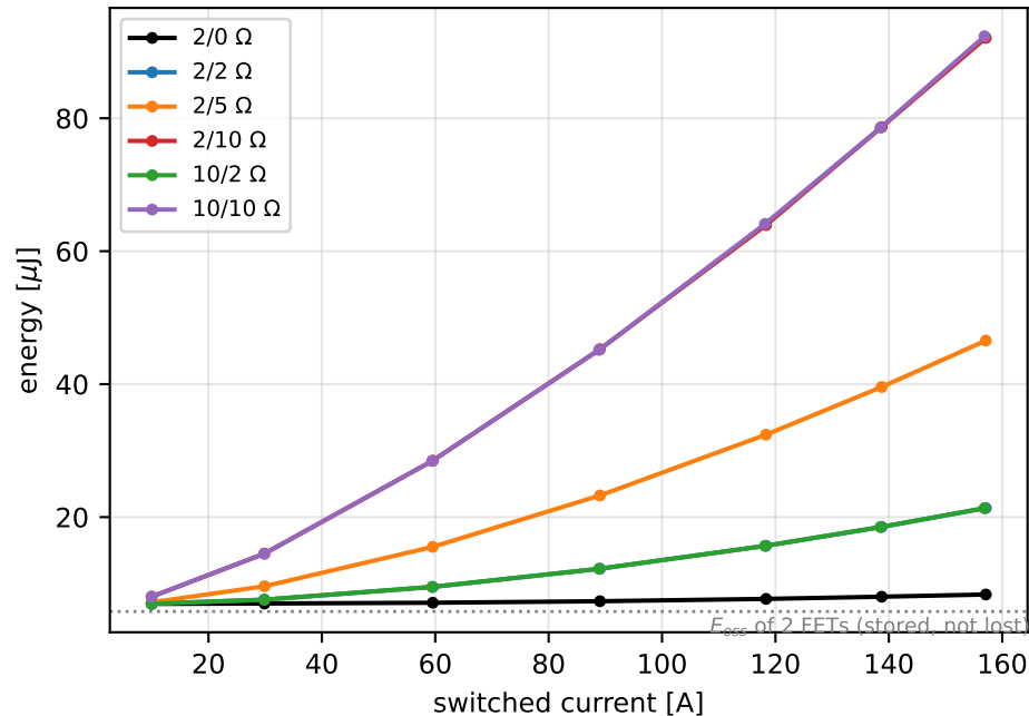
turn-off energy
