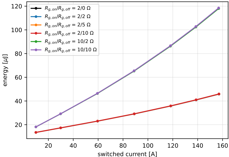
turn-on energy (2 x EPC2361, 75 V)
