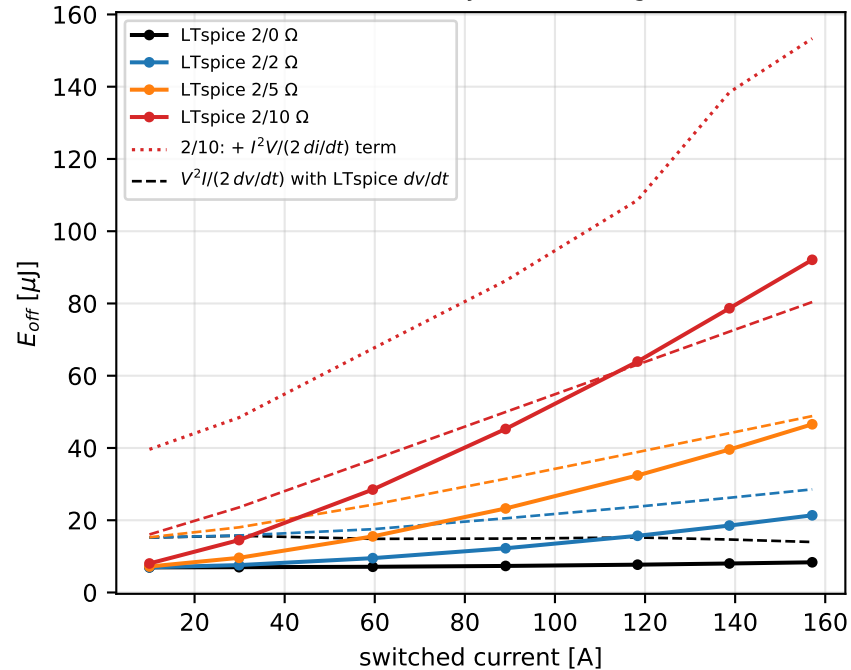
turn-off: dv/dt term only, valid when gate-driven
