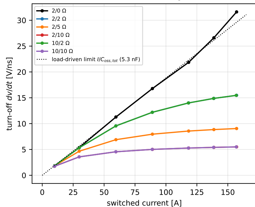
turn-off dv/dt : load-driven vs gate-driven
