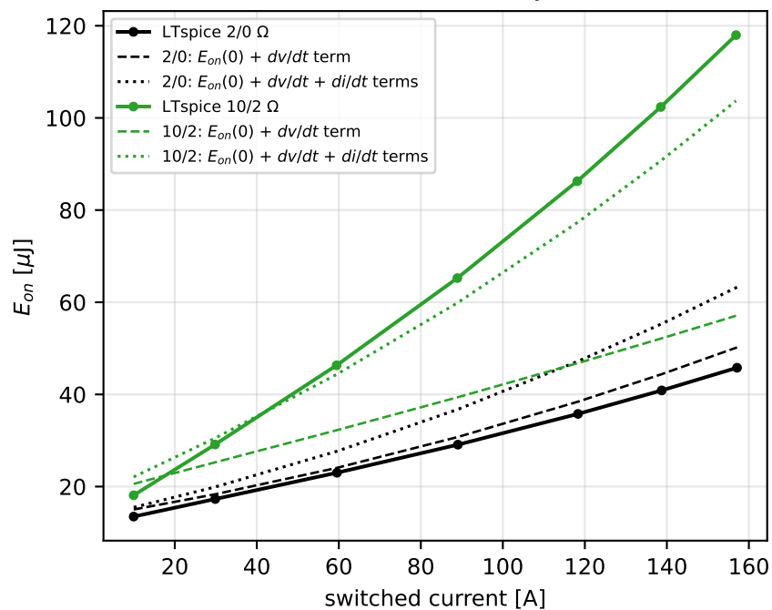
turn-on: di/dt term needed only when slow
