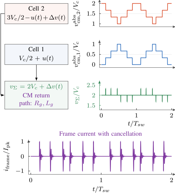
FIGURE 11. Nonideal two-cell common-mode cancellation over two switching periods. Small transition misalignment produces narrow residuals in v_{\Sigma} ( t_d/T_{sw} = 0.003 , t_r/T_{sw} = 0.004 ). Their polarities follow the three rising and three falling cell-voltage transitions; unequal dv/dt can also produce residuals. The lower plot shows damped frame current with cancellation, normalized to its own peak I_{pk} . For equal winding-to-frame capacitances C_g and a shared frame-to-ground return impedance R_g + sL_g , I_{frame}(s)/V_{\Sigma}(s) = sC_g/(1 + 2R_gC_g s + 2L_gC_g s^2) . The illustrative resonance has f_0/f_{sw} = 65 and damping ratio \zeta = 0.22 . Each residual excites alternating-polarity current ringing. This lumped-model illustration excludes shaft charging and bearing-film breakdown; it is not a bearing-discharge prediction.
