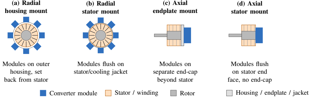
FIGURE 7. Physical integration options for SPB-compatible converter modules on a radial-flux machine, following the four-category taxonomy of [79]: (a) radial housing mount, (b) radial stator mount, (c) axial endplate mount, and (d) axial stator mount, each shown in whichever radial or axial cross-section most clearly conveys its mounting geometry.
