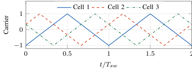
FIGURE 8. Uniform carrier interleaving for N = 3 , with phase offsets 0 , 2\pi/3 , and 4\pi/3 . Analytically generated triangular carriers.
