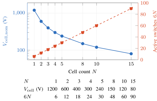
FIGURE 13. Cell-count scaling for a 1200-V dc link: nominal cell voltage V_{\text{cell,nom}} = V_{\text{dc}}/N (blue circles, left logarithmic axis) and active switch positions 6N (red squares, right linear axis). The table gives the values at each design point. Illustrative device classes include 1700–2000-V SiC for N = 1 , 650-V GaN/SiC for N = 3 , and 100-V GaN or silicon MOSFETs for N = 15 , subject to the required blocking-voltage margin. Device parallelization is excluded.
