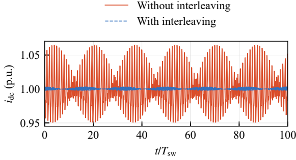
FIGURE 9. Analytical steady-state shared dc-link current for three identical SPB cells with ideal natural SPWM over one fundamental period. Parameters are M = 0.85 , power-factor angle 20^\circ , f_{sw}/f_1 = 100 , L_b C/T_{sw}^2 = 0.85 , and R_b C/T_{sw} = 2.5 . Exact switching-interval Fourier integrals are propagated through (12), retaining 8000 fundamental harmonics. Both averages are 1 p.u.; ripple RMS is 0.0281 p.u. without interleaving and 0.00126 p.u. with uniform interleaving. These are ideal-model predictions, not measurements.
