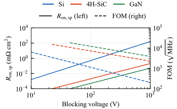
FIGURE 2. Ideal one-dimensional unipolar specific on-state resistance R_{on,sp} (solid, left axis) and the resulting high-frequency figure of merit FOM = 1/\sqrt{R_{on,sp}C_{oss,sp}} (dashed, right axis), in \sqrt{\text{MHz}} – the product R_{on,sp}C_{oss,sp} is an area-independent RC time constant, versus blocking voltage for Si, 4H-SiC, and GaN.
