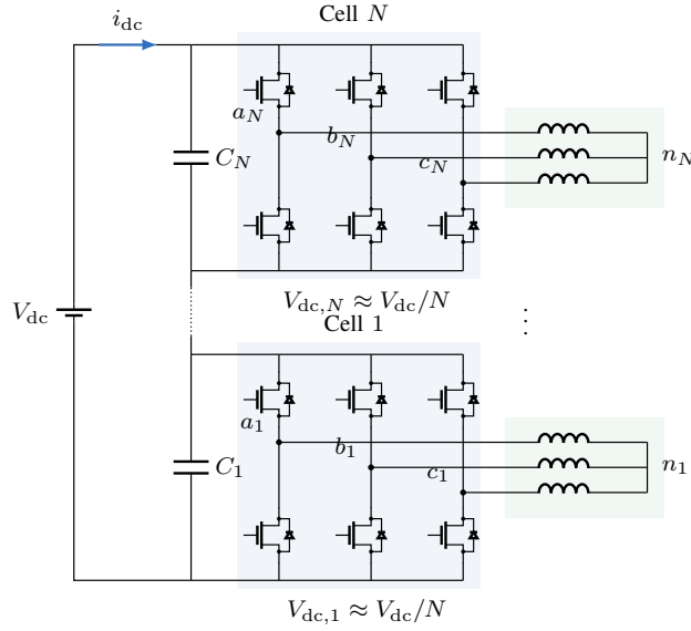
FIGURE 5. Switch-level realization of the SPB dc-ac stage for two representative cells (Cell 1 and Cell N ; cells 2, \dots, N-1 elided). The common series current i_{dc} (2) flows through every cell, giving each cell the dc-side power p_{dc,k} = V_{dc,k} i_{dc} (3).
