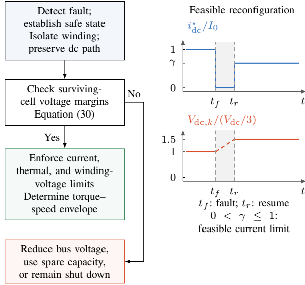
FIGURE 15. Post-fault feasibility assessment with illustrative waveforms for the feasible branch. The dc-current command is temporarily set to zero and restored to \gamma I_0 , subject to operating limits. For a fixed bus, changing from three to two active cells raises the balanced surviving-cell voltage from 1 to 1.5 p.u. (400 to 600 V for a 1200-V bus). Shading marks the protection/reconfiguration interval; the dashed voltage connection indicates a change of steady-state level, not a predicted capacitor-voltage trajectory. Current derating does not remove the increased blocking-voltage requirement.
