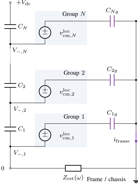
FIGURE 10. Lumped common-mode equivalent of the SPB stack. Series dc-link capacitors C_k establish the rail offsets V_{-,k} ; each voltage source represents v_{cm,k}^{loc} = (v_{aN_k} + v_{bN_k} + v_{cN_k})/3 . The group-to-frame capacitance C_{kg} couples this local source and its rail offset to the chassis. Z_{ret}(\omega) represents the installation-dependent return path to the dc reference, not an assumed galvanic bond. Differential-mode winding circuits and the rotor/bearing network are omitted.
