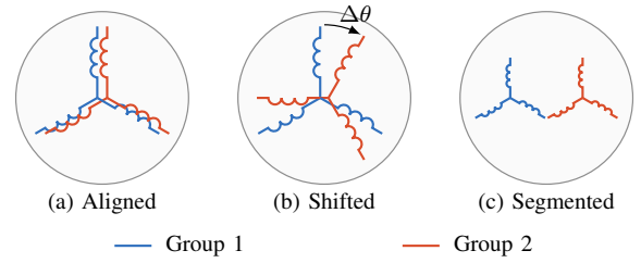
FIGURE 6. Schematic comparison of winding-group spatial arrangements, each coil marking one phase axis of winding group 1 (blue) or group 2 (red): (a) aligned groups (parallel phase axes), (b) spatially shifted groups (offset by \Delta\theta ), and (c) physically segmented stator modules.
