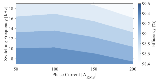
FIGURE 14. Measured inverter efficiency along with RMS phase current and switching frequency at V_{dc} = 1200\text{ V} .
