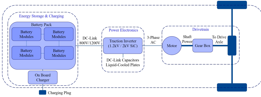
FIGURE 1. Schematic of the HDV traction system with battery, traction inverter, motor, and gearbox driving the axle.
