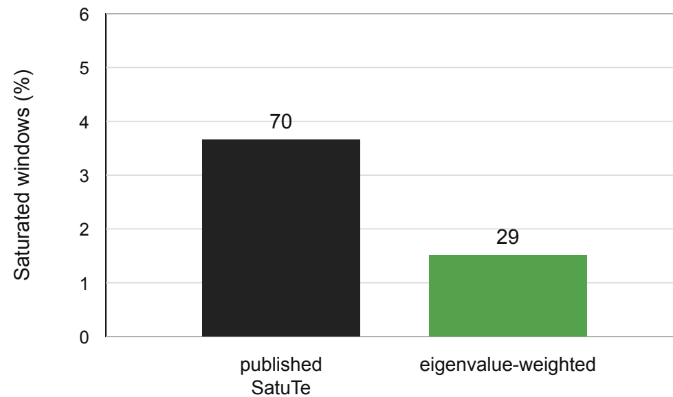
16S rRNA 3D tree - yeast
