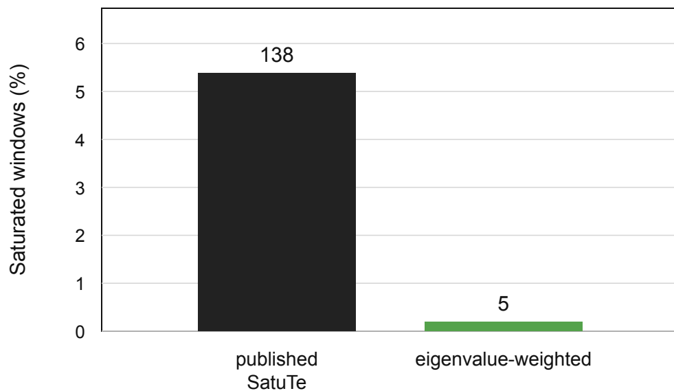
protein 2D tree - Eukaryota
