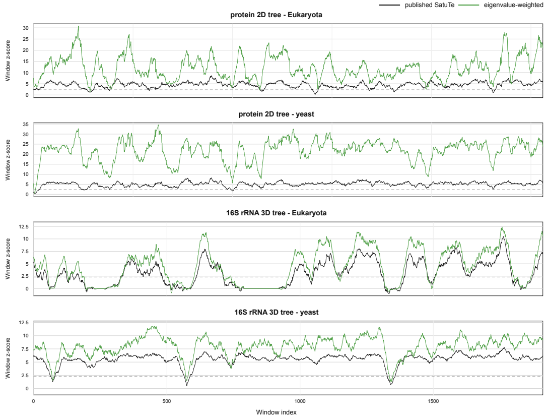
Figure 6: Independent eigenvalue-weighted sliding-window curves for the protein 2D and 16S rRNA 3D Tree-of-Life examples. The independent calculation compares the published SatuTe sliding-window score with the eigenvalue-weighted statistic on the same 36-site windows and target branches.
