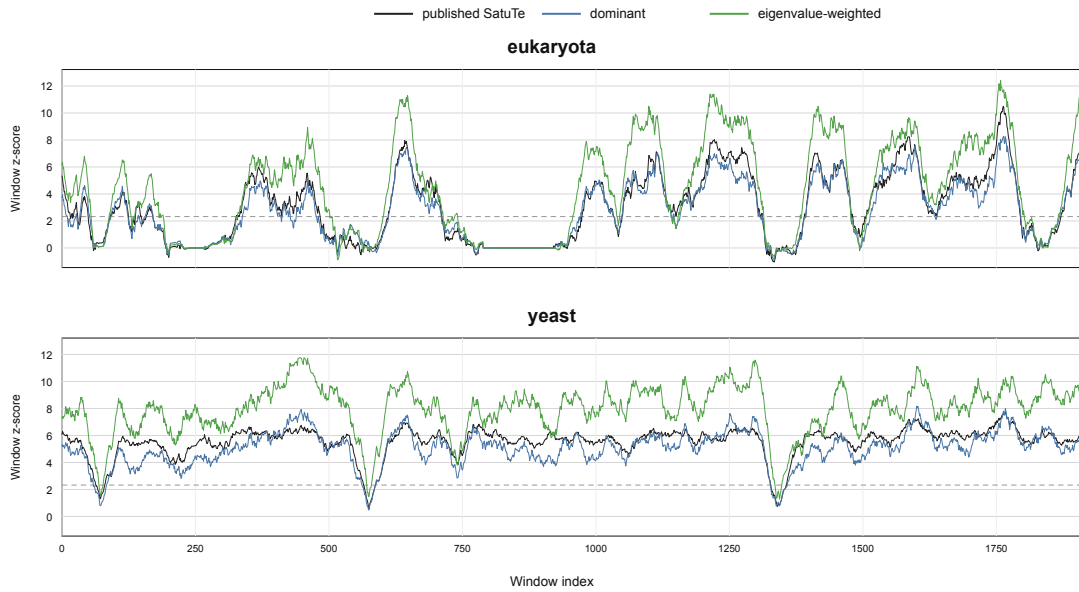
Figure 4: Published SatuTe and eigenvalue-weighted sliding-window curves for the 16S rRNA Tree-of-Life example. The curves compare the manuscript SatuTe rerun with the native dominant calculation and the eigenvalue-weighted statistic for the branches leading to Eukaryota and yeast.
