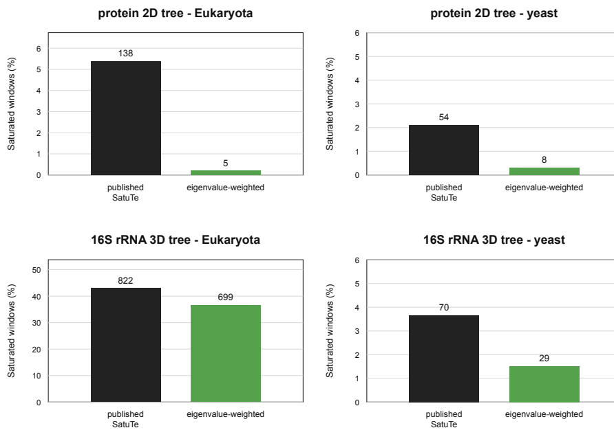
Figure 7: Saturated-window counts in the independent biological comparison. Counts are shown for the branch leading to Eukaryota and the branch leading to yeast in the protein-based 2D tree and the 16S rRNA-based 3D tree.
