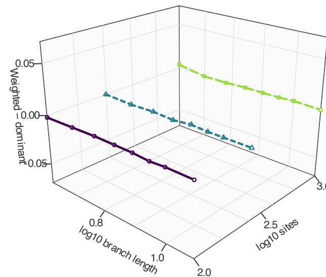
16-taxon internal branch True tree, fixed lengths
