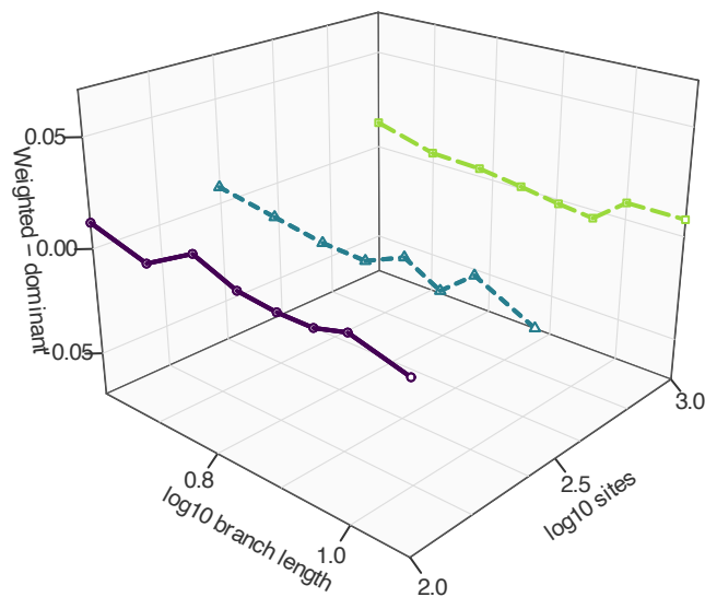
16-taxon internal branch ML tree
