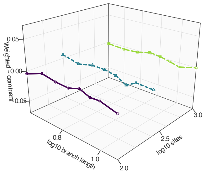
16-taxon internal branch True topology, ML lengths
