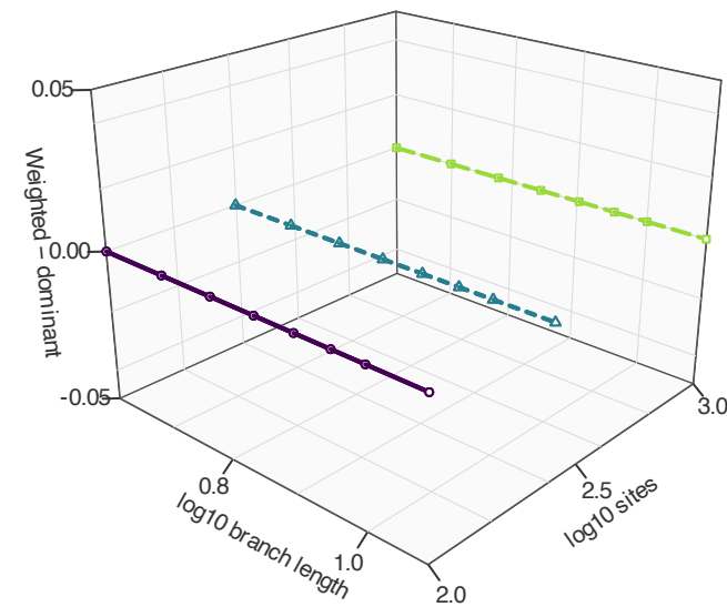
16-taxon internal branch True tree, fixed lengths
