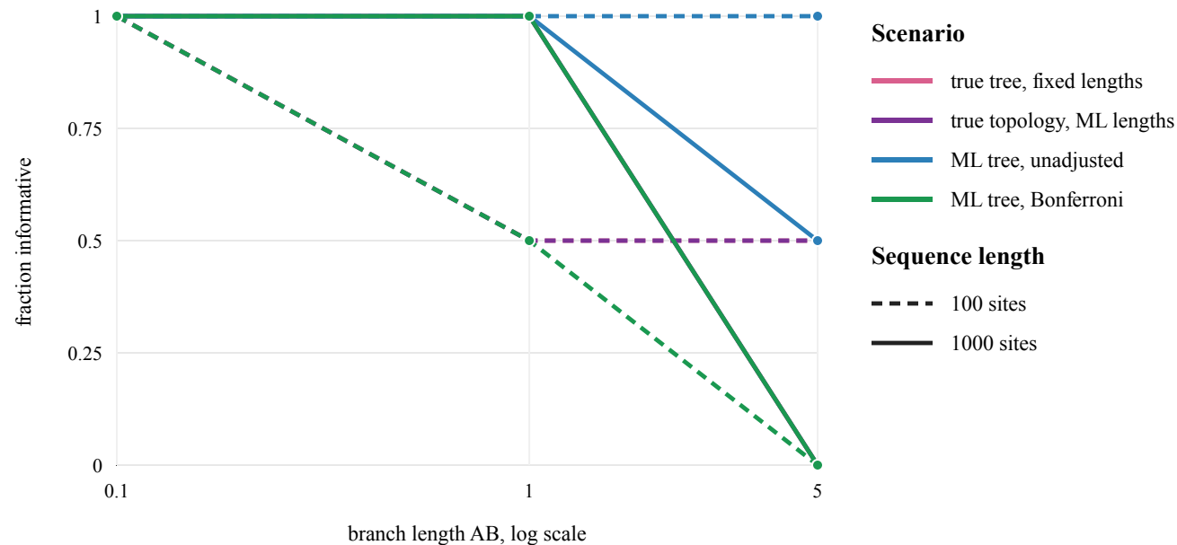
b) 16-taxon internal branch
