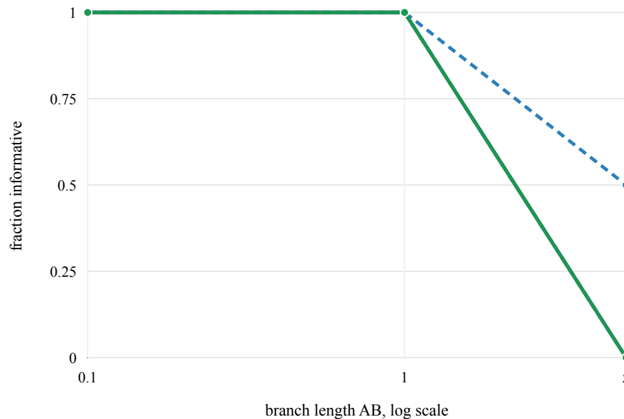
a) five-taxon external branch
