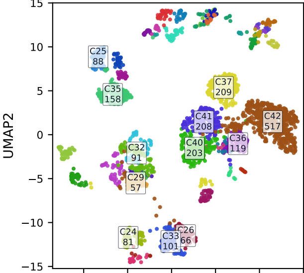
Adaptive diffusion recomputed NNLS branch-time TBS: 43 clusters, 12 clusters >= 50 cells
