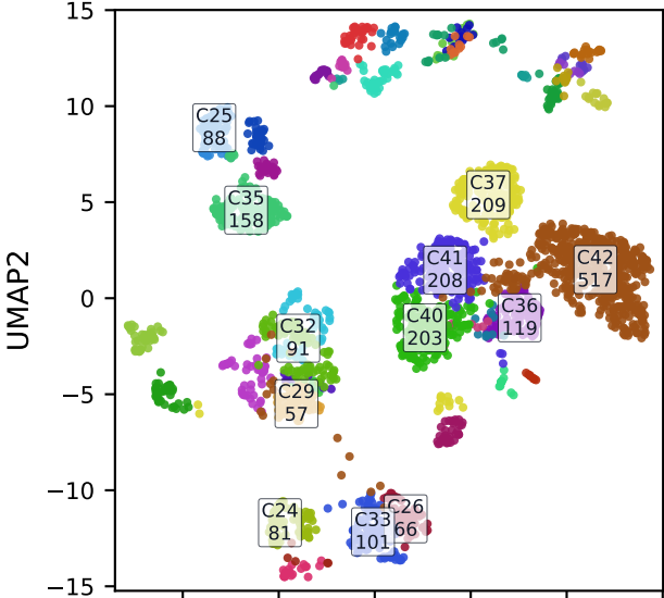
Adaptive diffusion raw-linkage branch-time diagnostic TBS: 41 clusters, 12 clusters >= 50 cells
