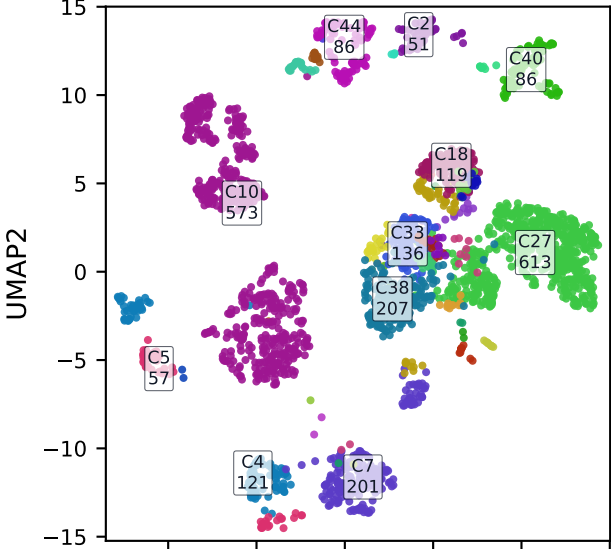
Recomputed NNLS branch-time TBS: 45 clusters, 11 clusters >= 50 cells
