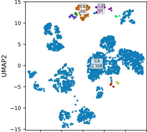
Adaptive diffusion topology TBS: 43 clusters, 12 clusters >= 50 cells
