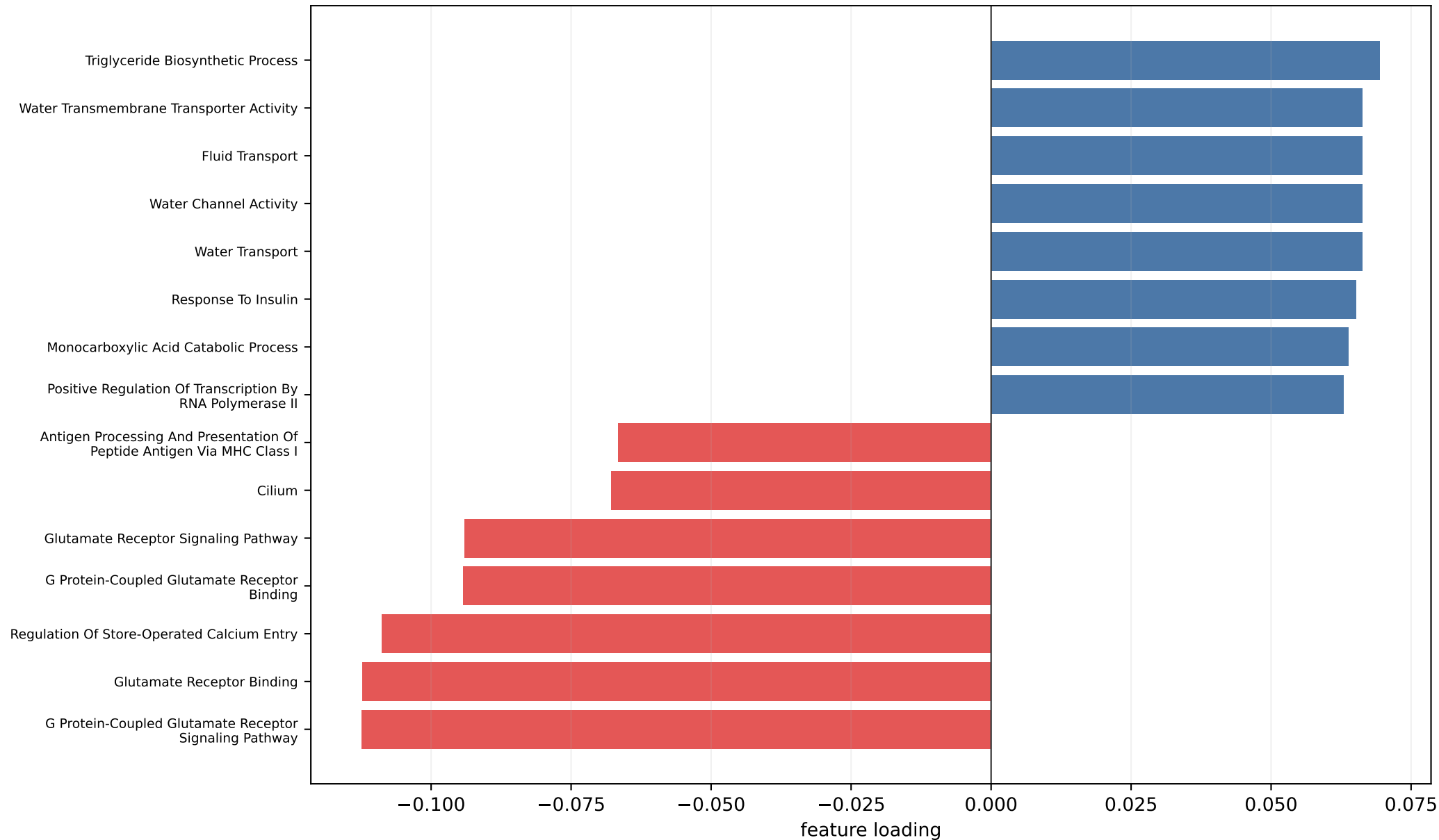
Rank 5: tfidf_adaptive_modes_53_80, mode 63 Top absolute GO-term loadings for this subspace axis
