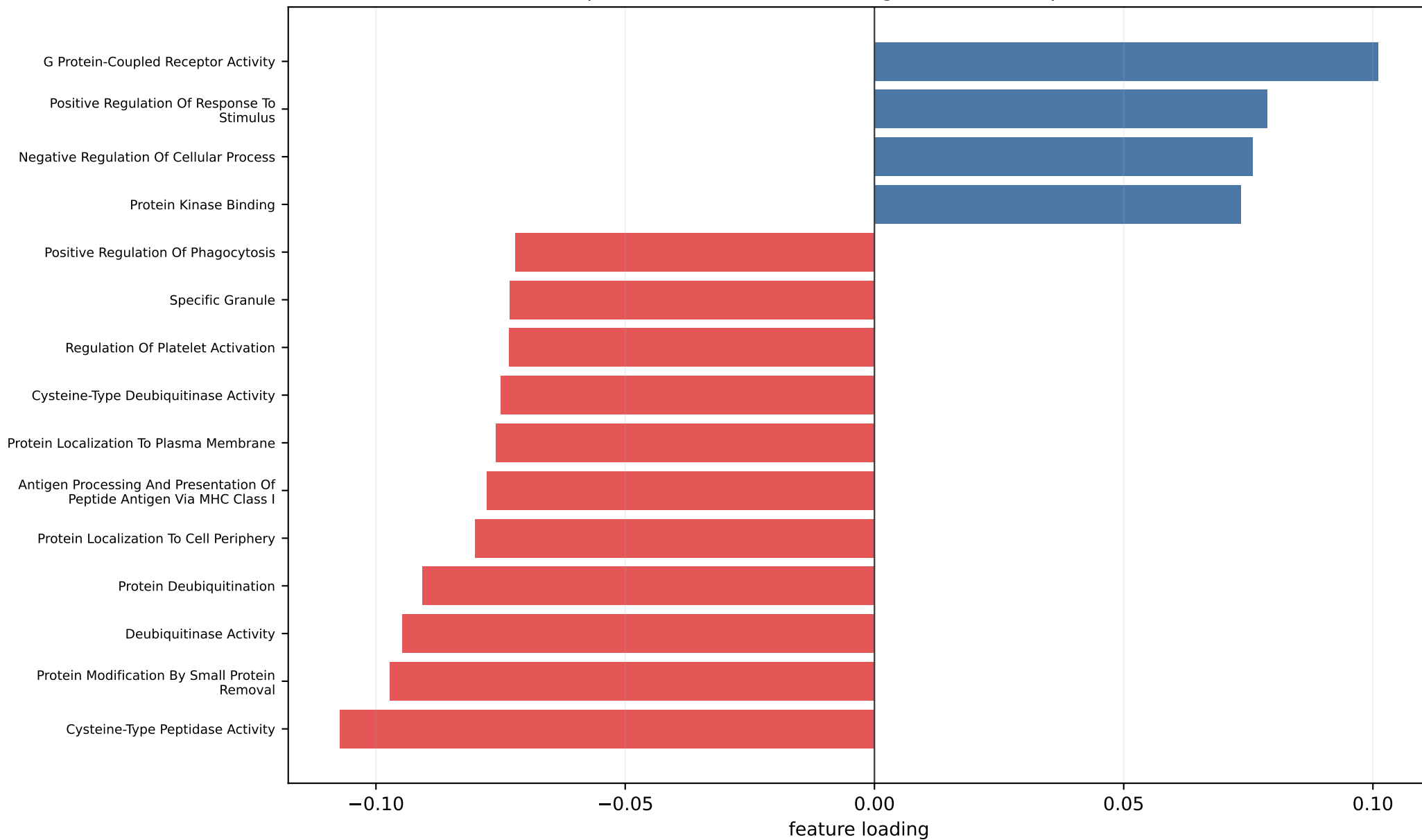
Rank 7: binary__adaptive_modes_56_80, mode 65 Top absolute GO-term loadings for this subspace axis
