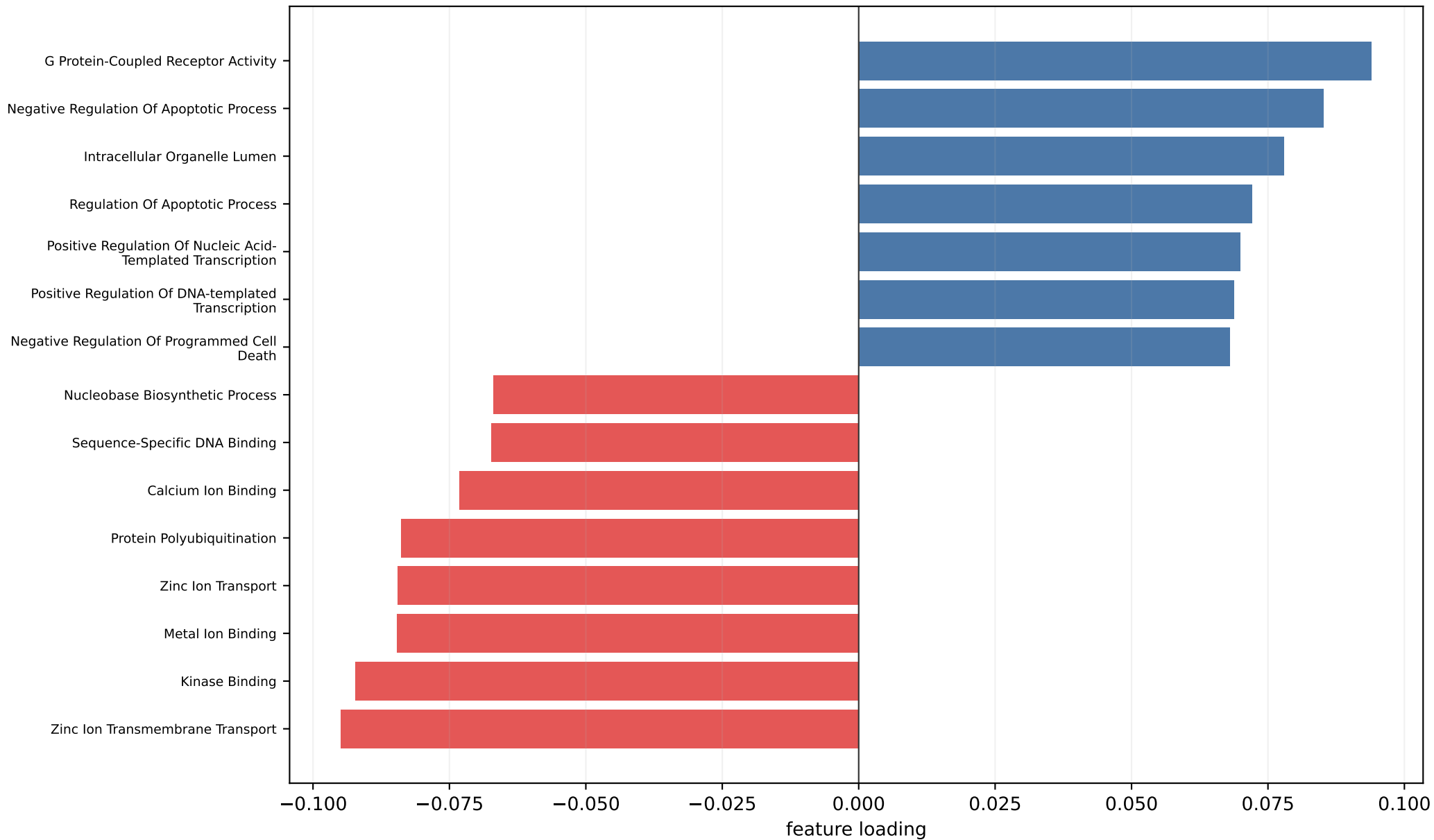
Rank 7: binary__adaptive_modes_56_80, mode 70 Top absolute GO-term loadings for this subspace axis
