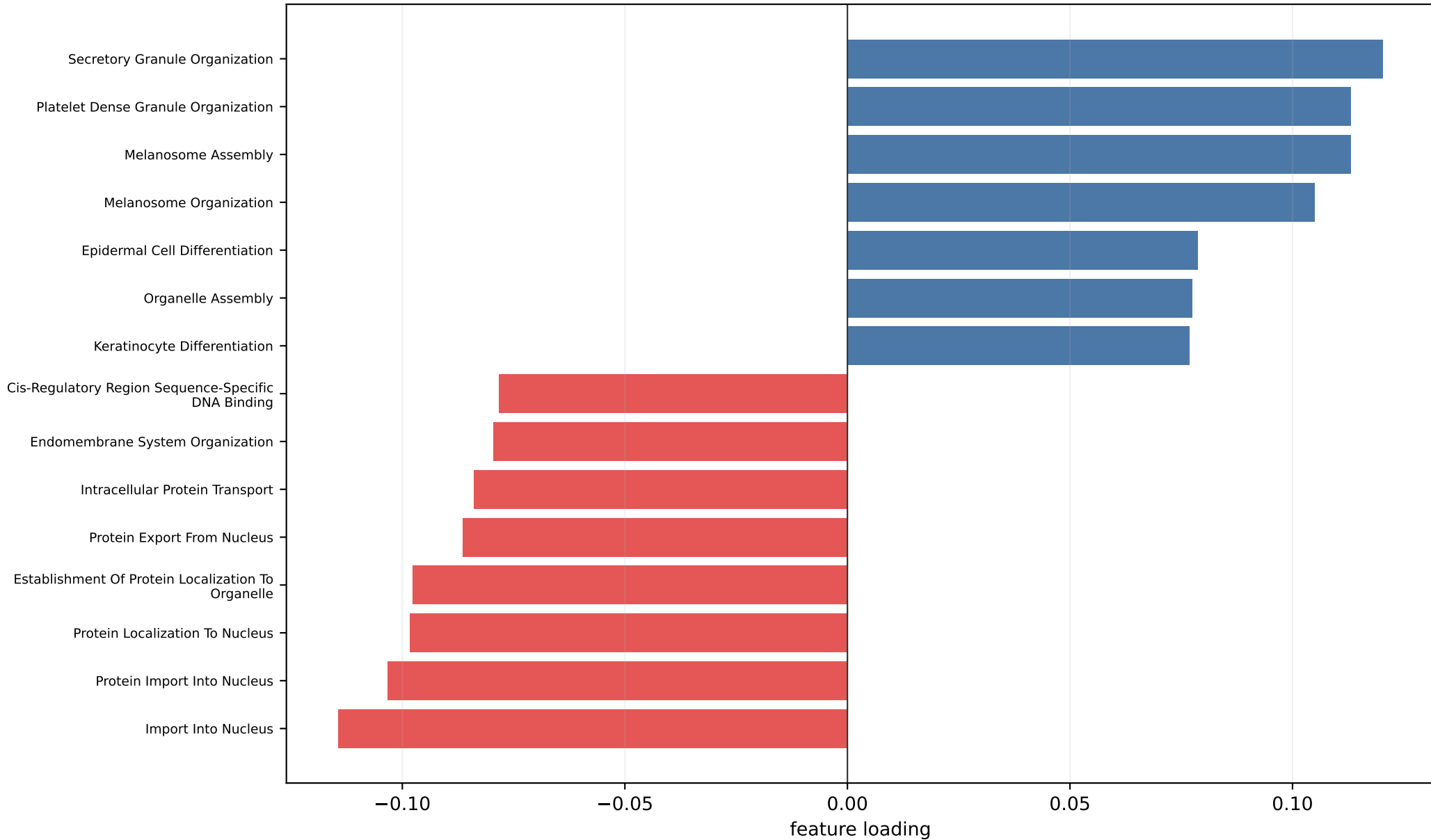
Rank 9: tfidf_adaptive_modes_20_31, mode 22 Top absolute GO-term loadings for this subspace axis
