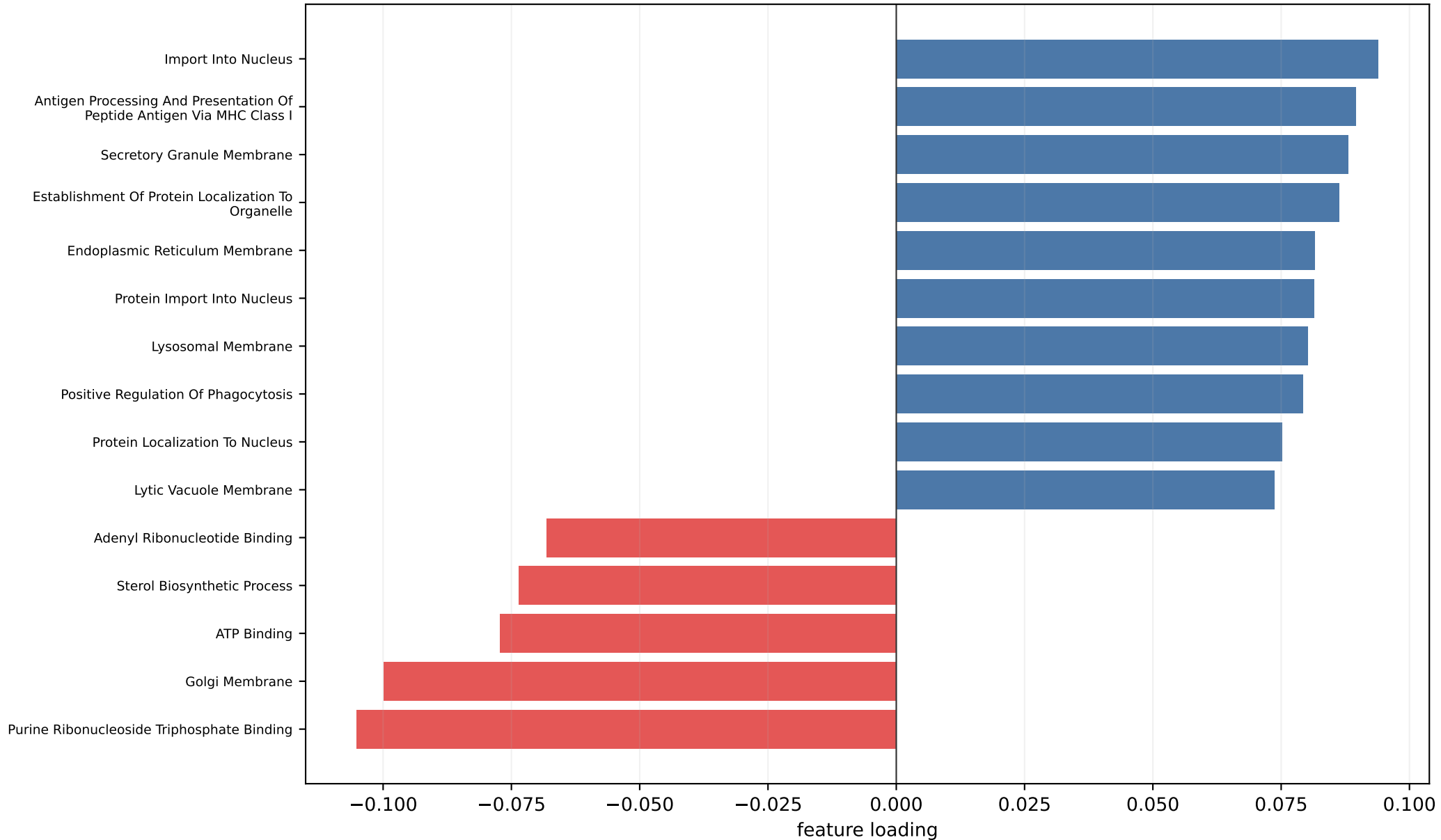
Rank 8: binary_adaptive_modes_41_55, mode 43 Top absolute GO-term loadings for this subspace axis
