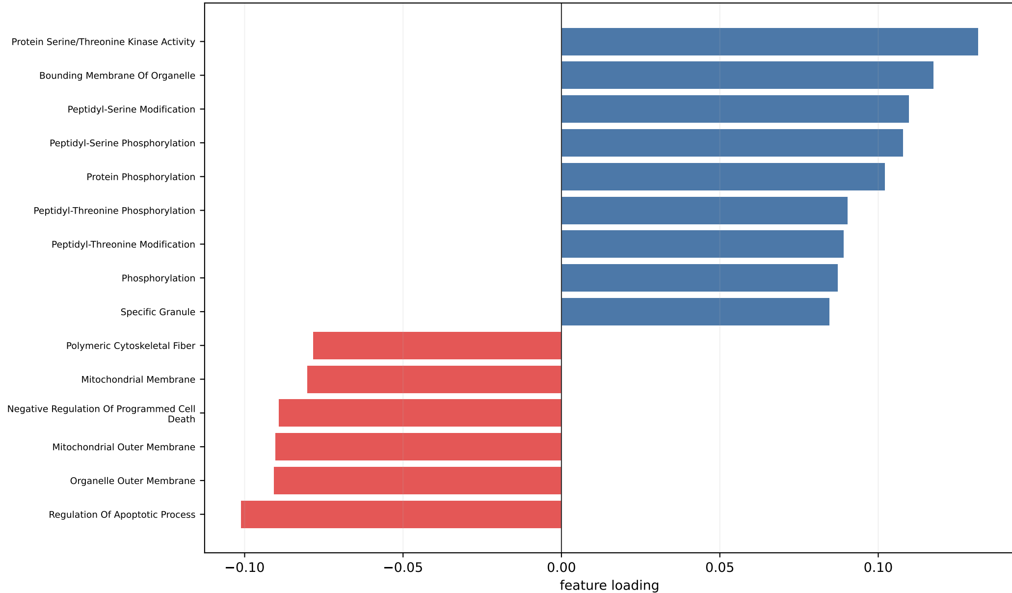
Rank 4: binary__adaptive_modes_12_21, mode 18 Top absolute GO-term loadings for this subspace axis
