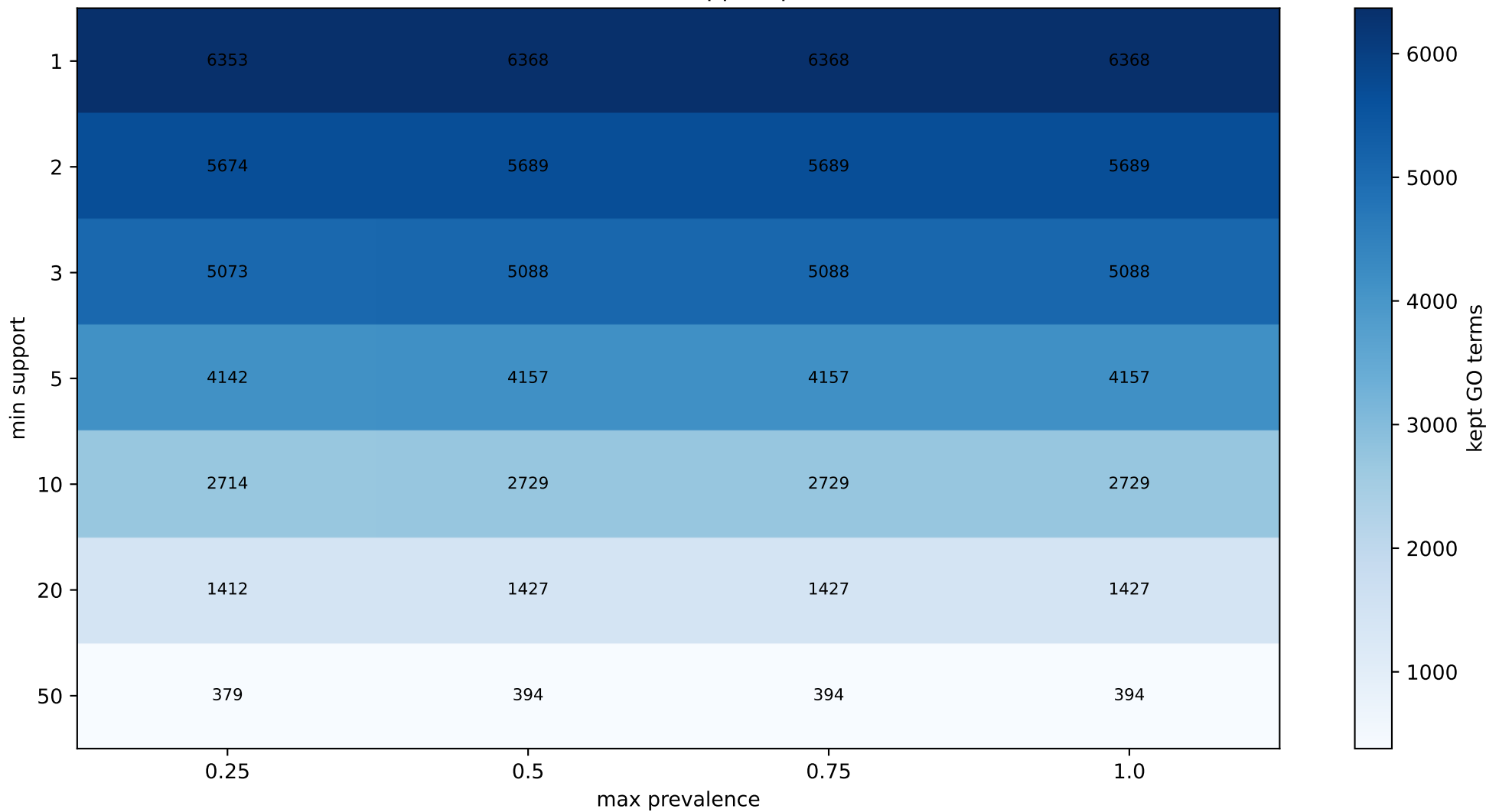
GO terms retained under support/prevalence filters
