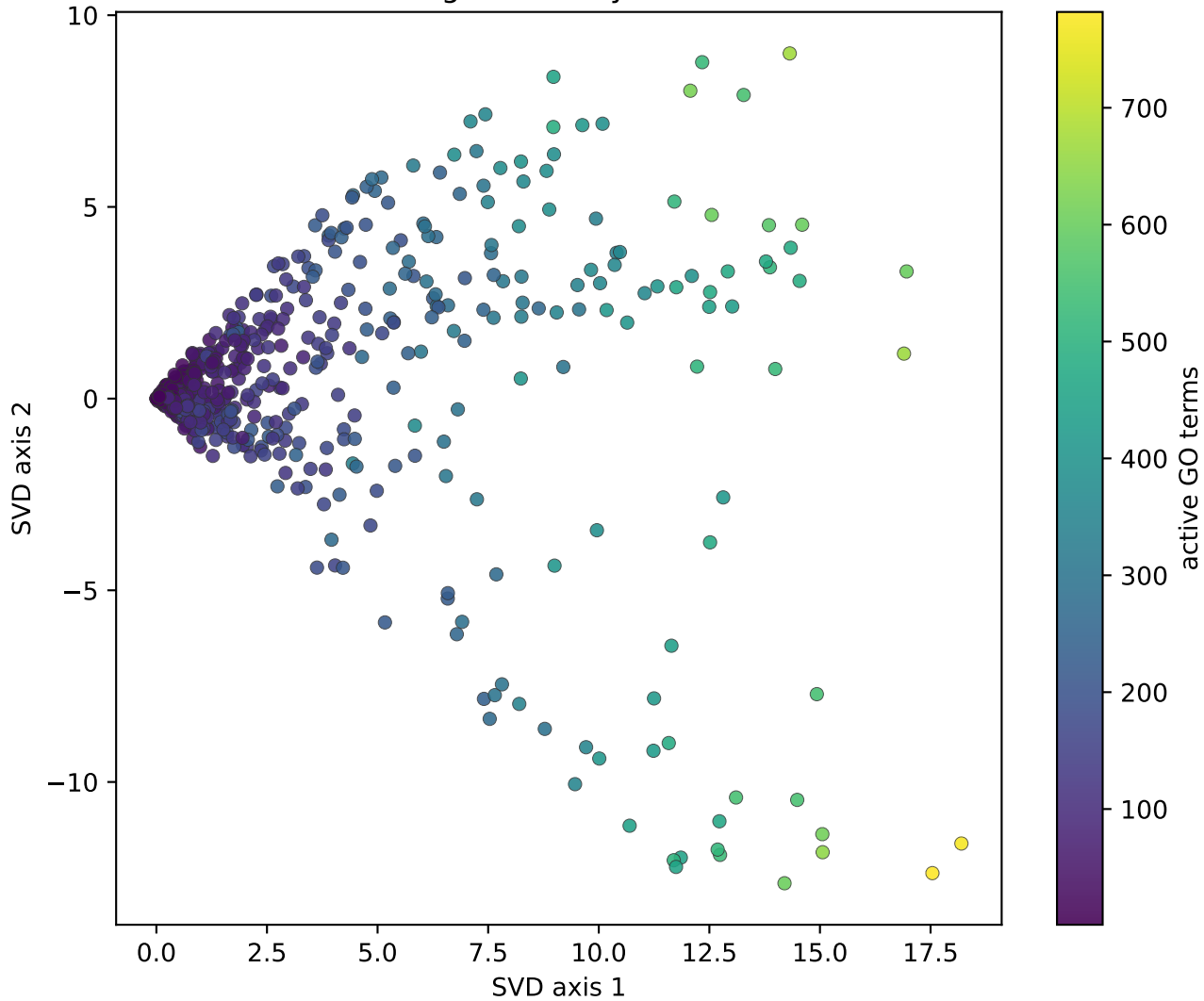
Gene embedding colored by annotation burden
