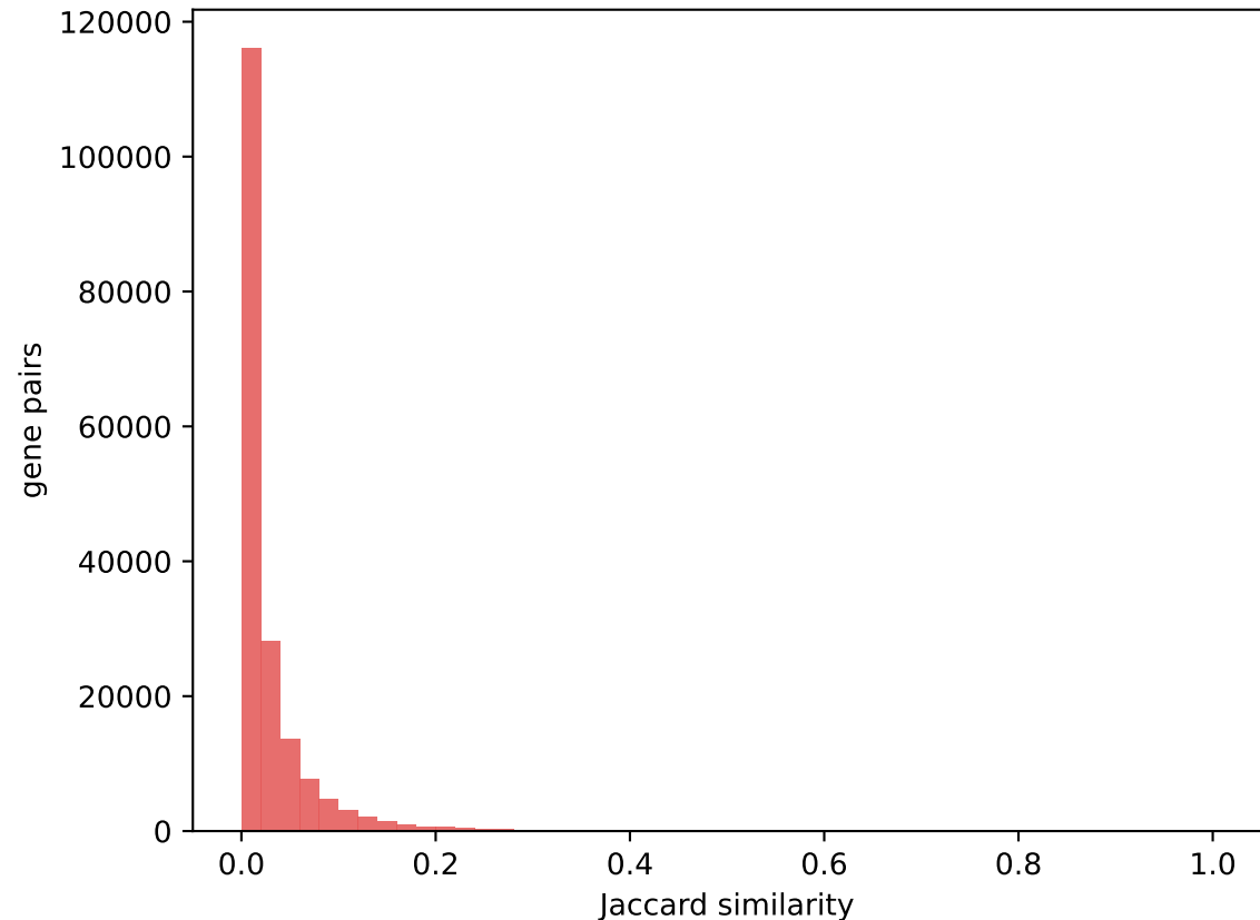
Pairwise gene Jaccard similarity
