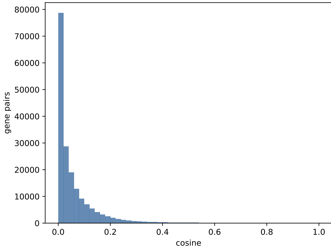
Pairwise gene cosine similarity
