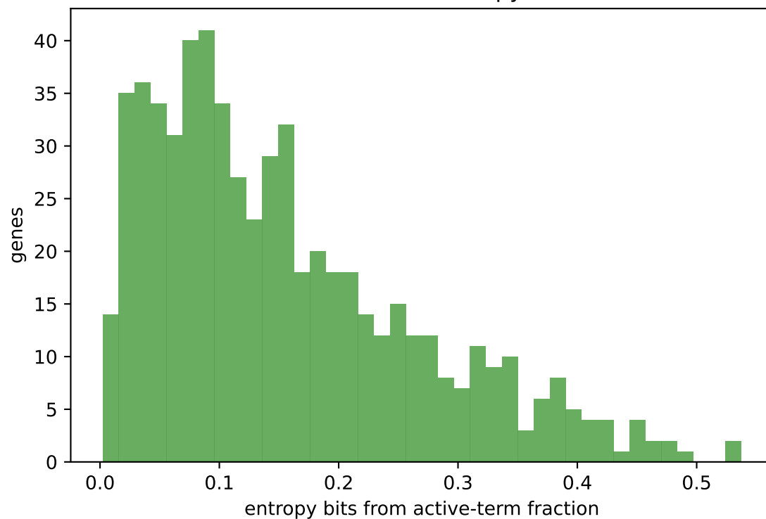
Gene row entropy
