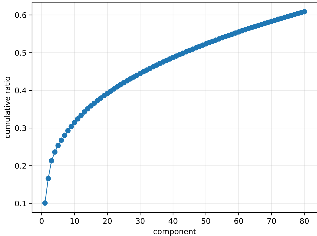
Cumulative SVD variance
