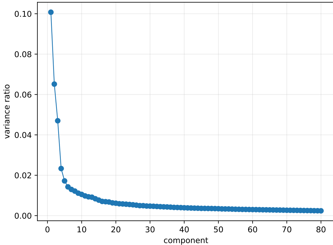
SVD explained variance ratio
