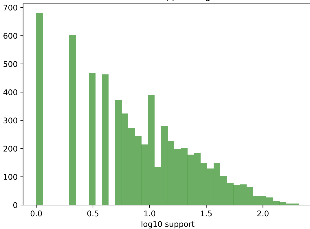
GO term support, log10
