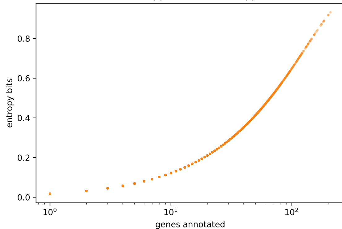
GO support versus entropy
