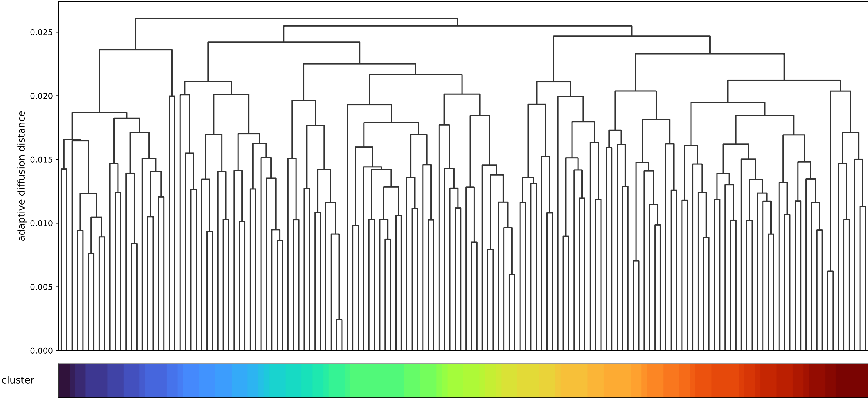
Rank 5: current adaptive diffusion cosine subspace, tfidf / adaptive_modes_63_80: tree with cluster assignments
