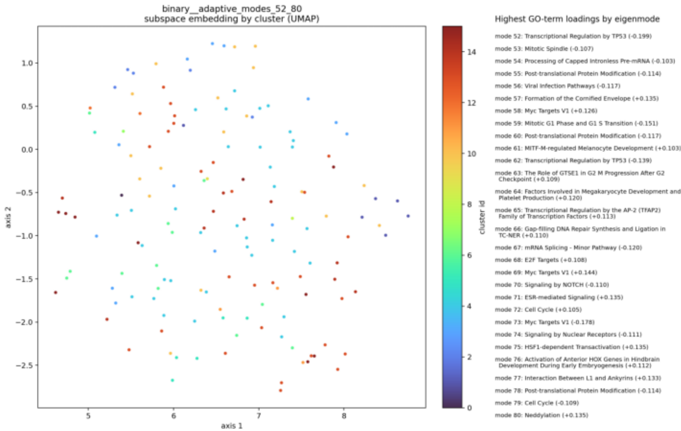
Subspace embedding
