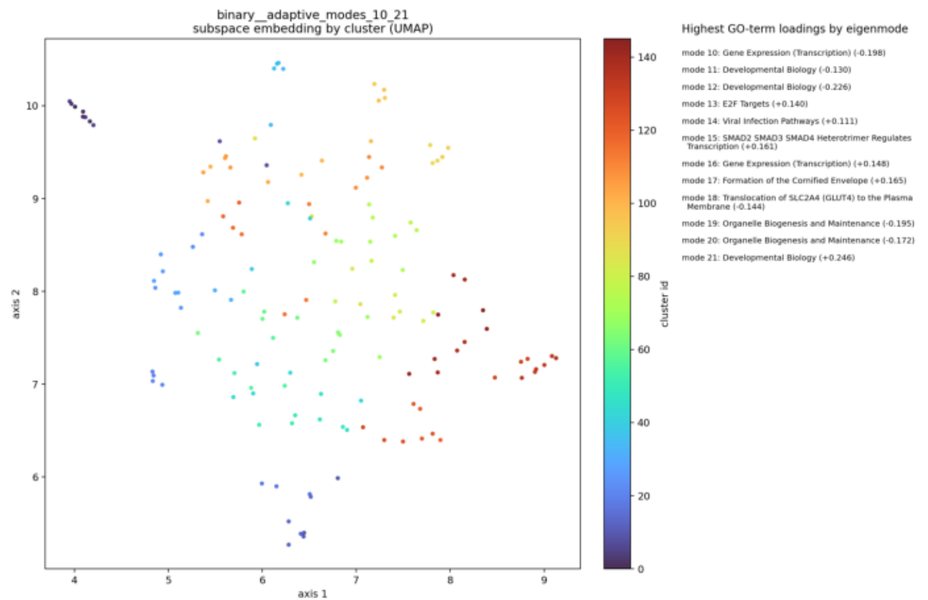
Subspace embedding
