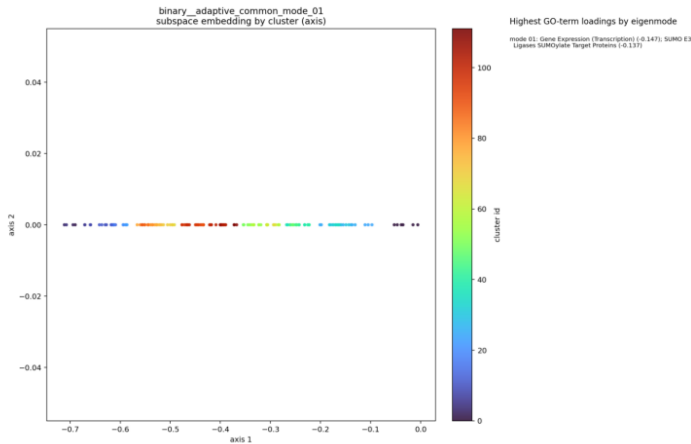
Subspace embedding
