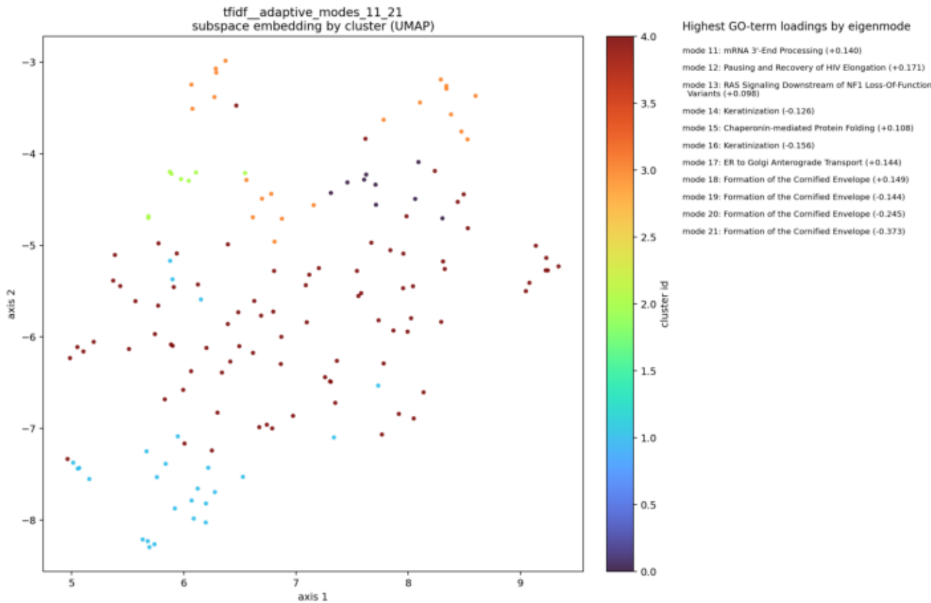
Subspace embedding
