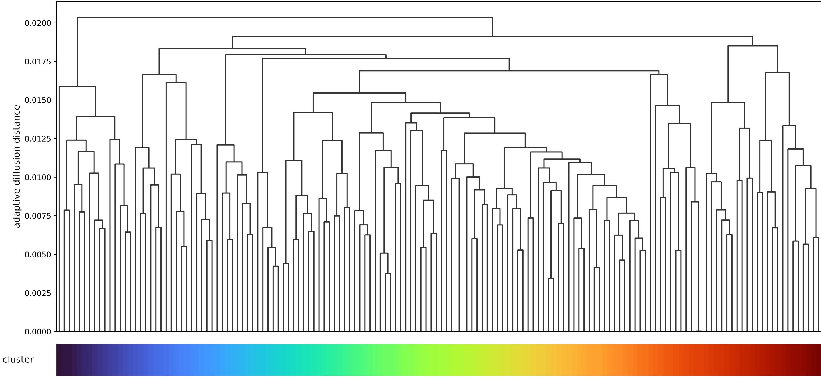
Rank 10: current adaptive diffusion cosine subspace, binary / adaptive_modes_22_51: tree with cluster assignments
