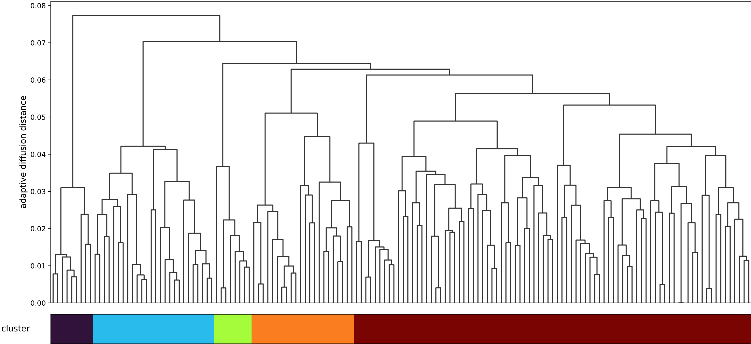
Rank 2: current adaptive diffusion cosine subspace, tfidf / adaptive_modes_11_21: tree with cluster assignments
