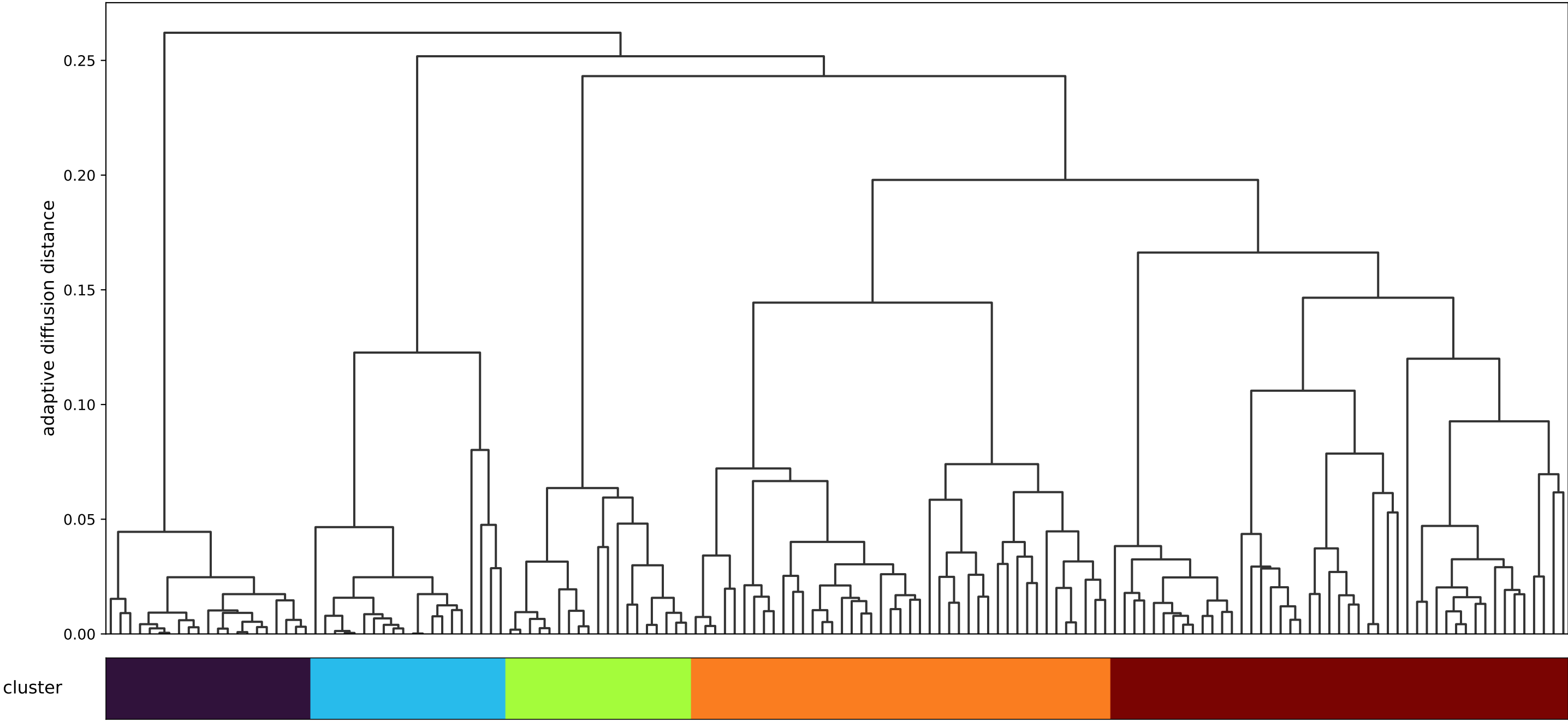
Rank 1: current adaptive diffusion cosine subspace, binary / adaptive_modes_02_05: tree with cluster assignments
