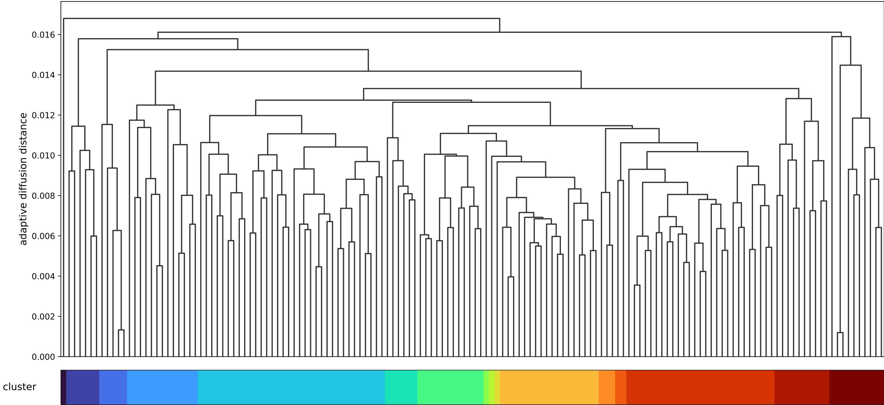
Rank 4: current adaptive diffusion cosine subspace, binary / adaptive_modes_52_80: tree with cluster assignments
