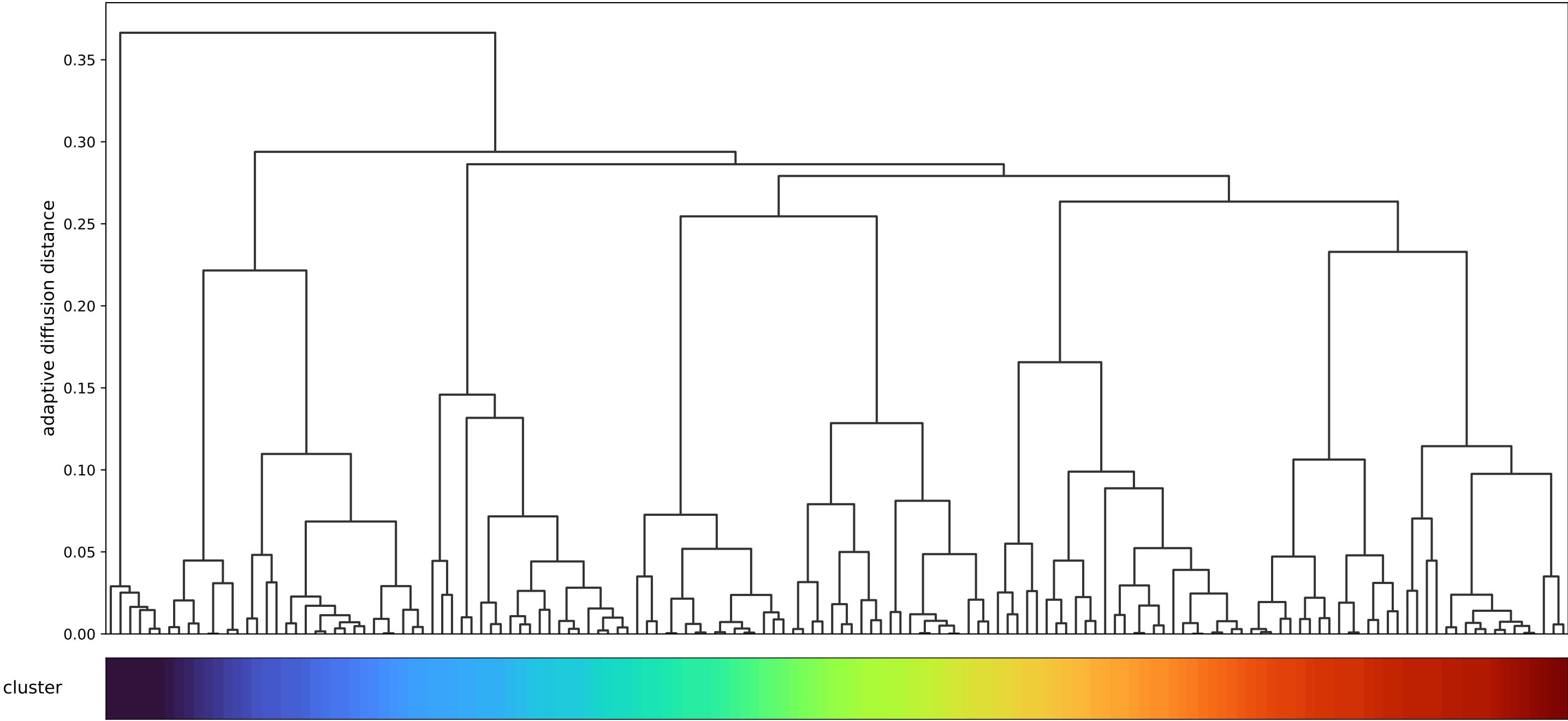
Rank 12: current adaptive diffusion cosine subspace, binary / adaptive_common_mode_01: tree with cluster assignments
