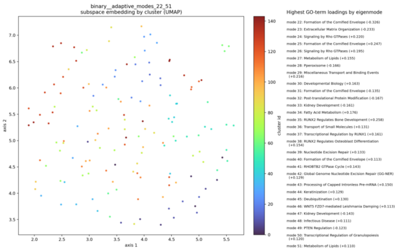
Subspace embedding
