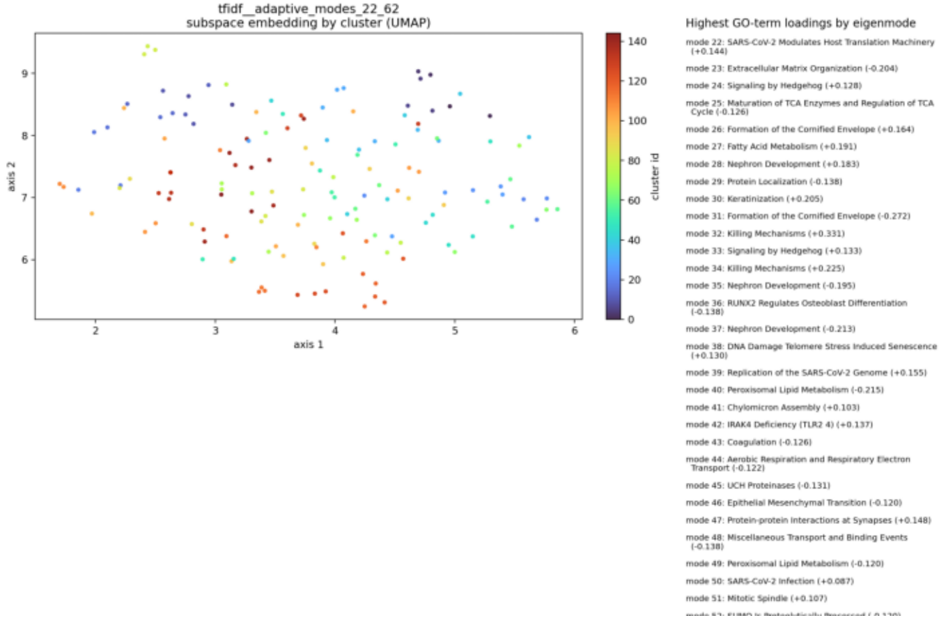
Subspace embedding
