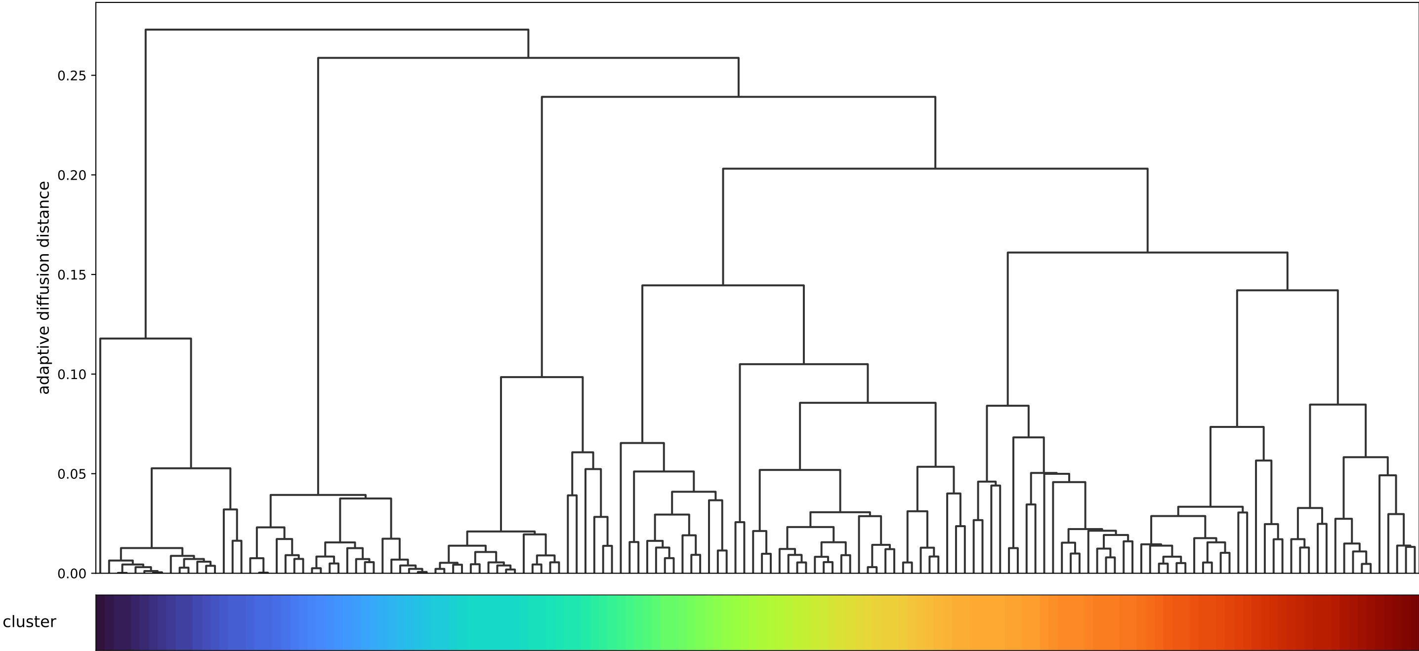
Rank 6: current adaptive diffusion cosine subspace, tfidf / adaptive_modes_02_05: tree with cluster assignments
