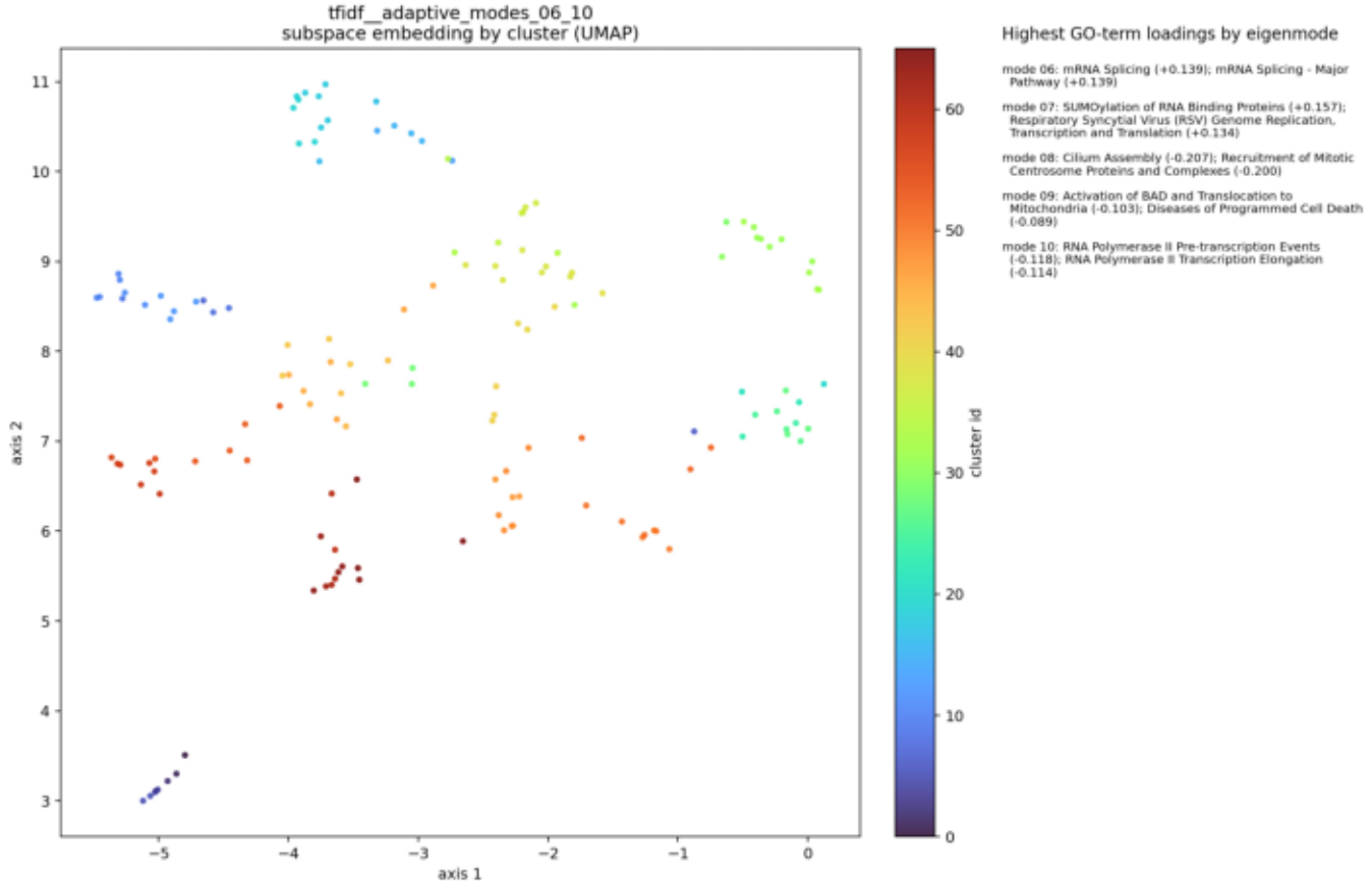
Subspace embedding
