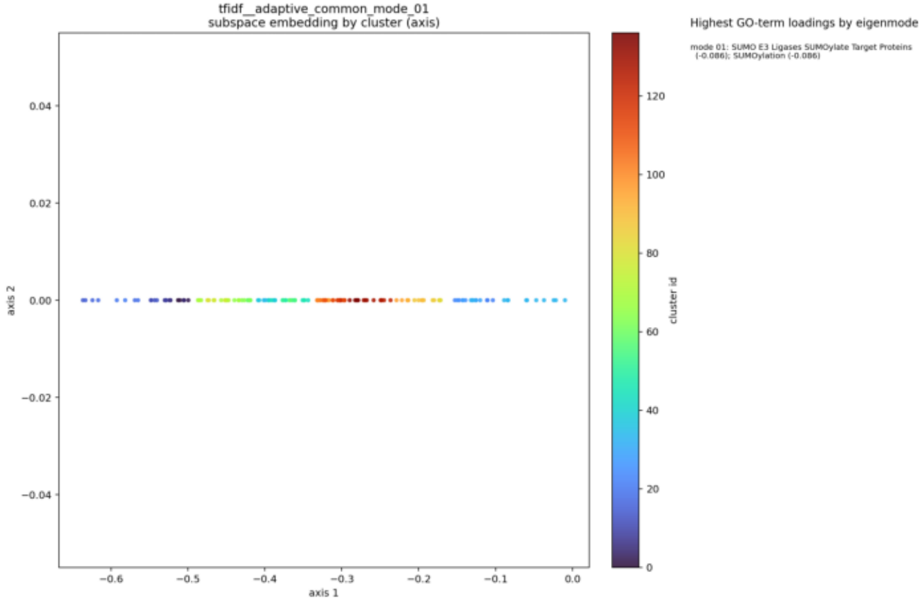
Subspace embedding
