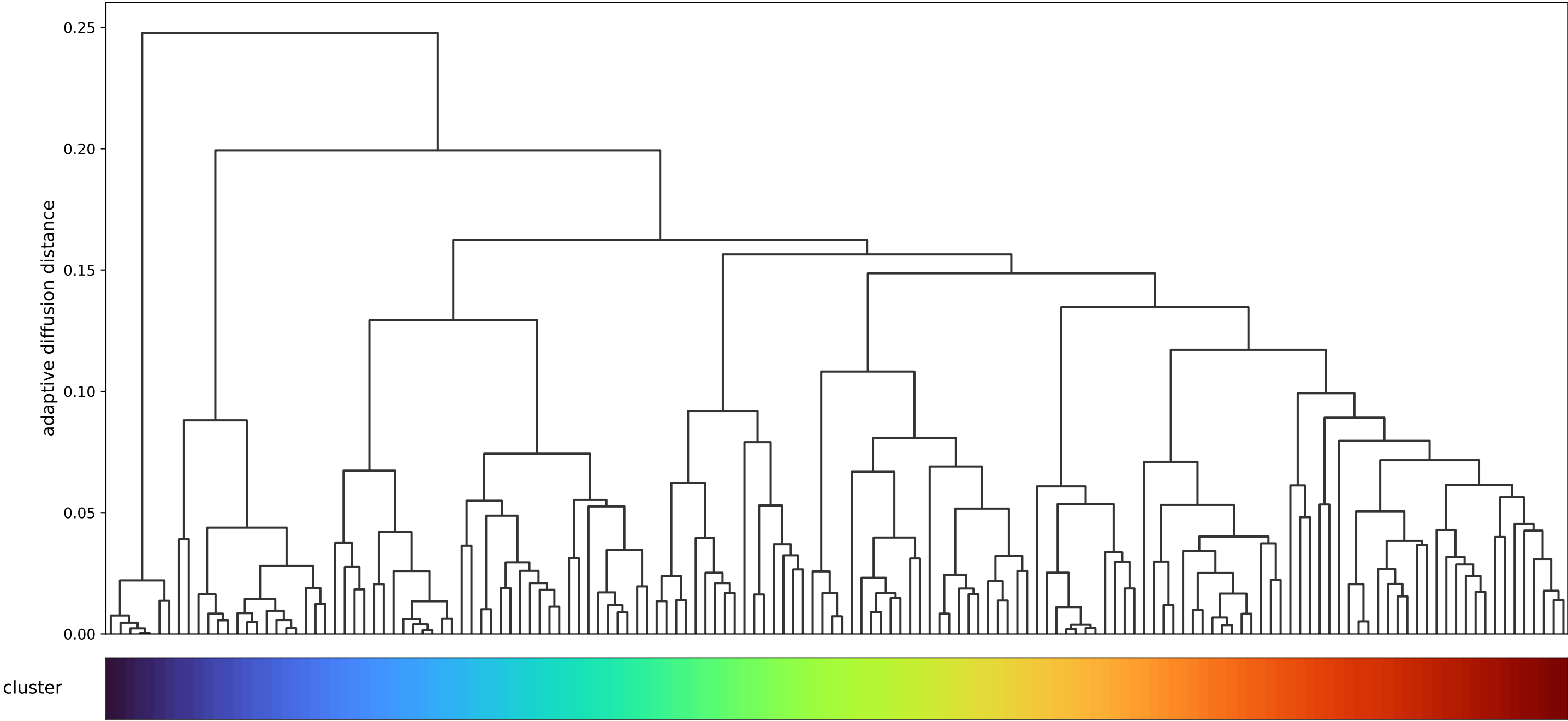
Rank 7: current adaptive diffusion cosine subspace, binary / adaptive_modes_06_09: tree with cluster assignments
