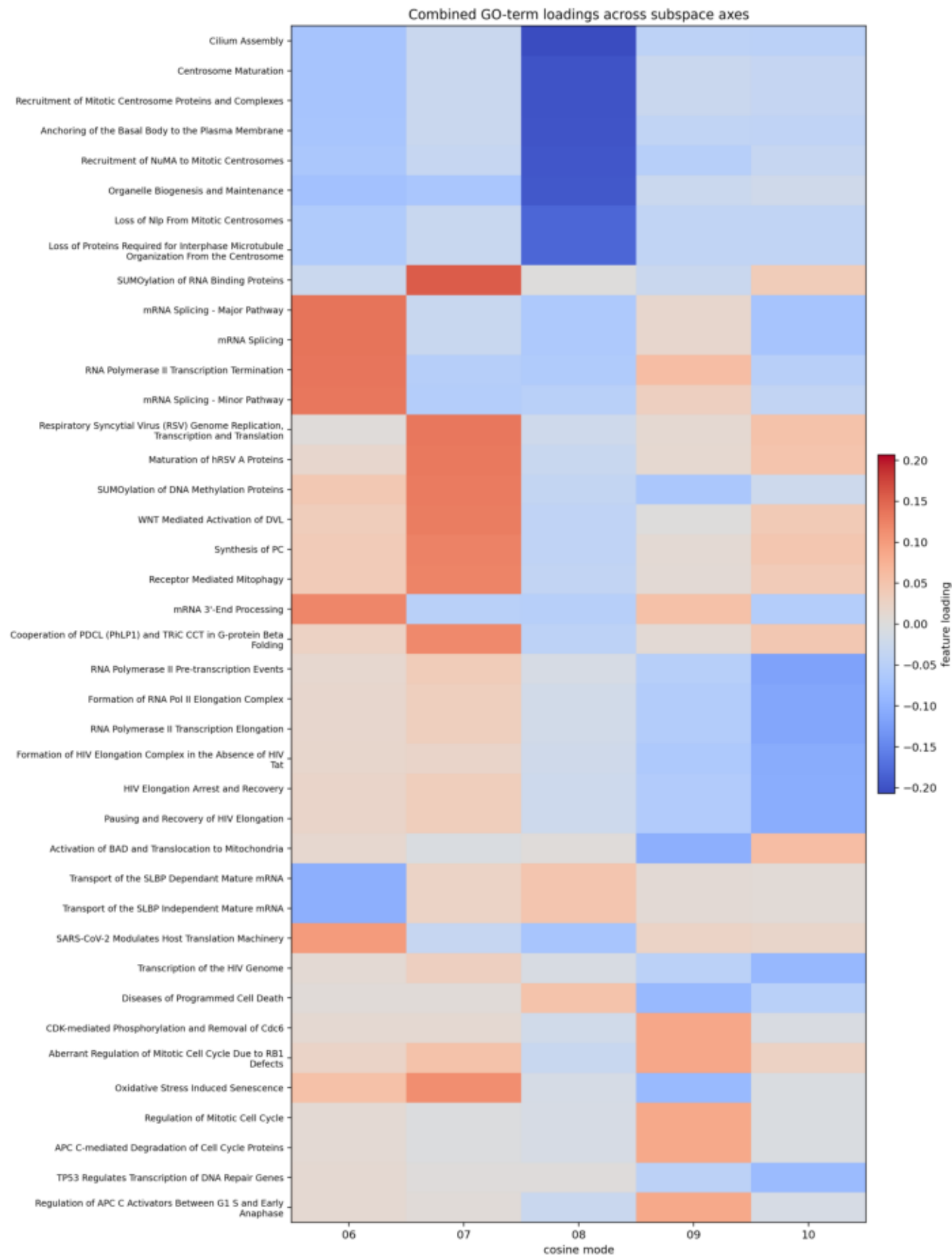
Rank 3: tfidf / adaptive_modes_06_10 Combined signed GO-term feature loadings across subspace eigenmodes
