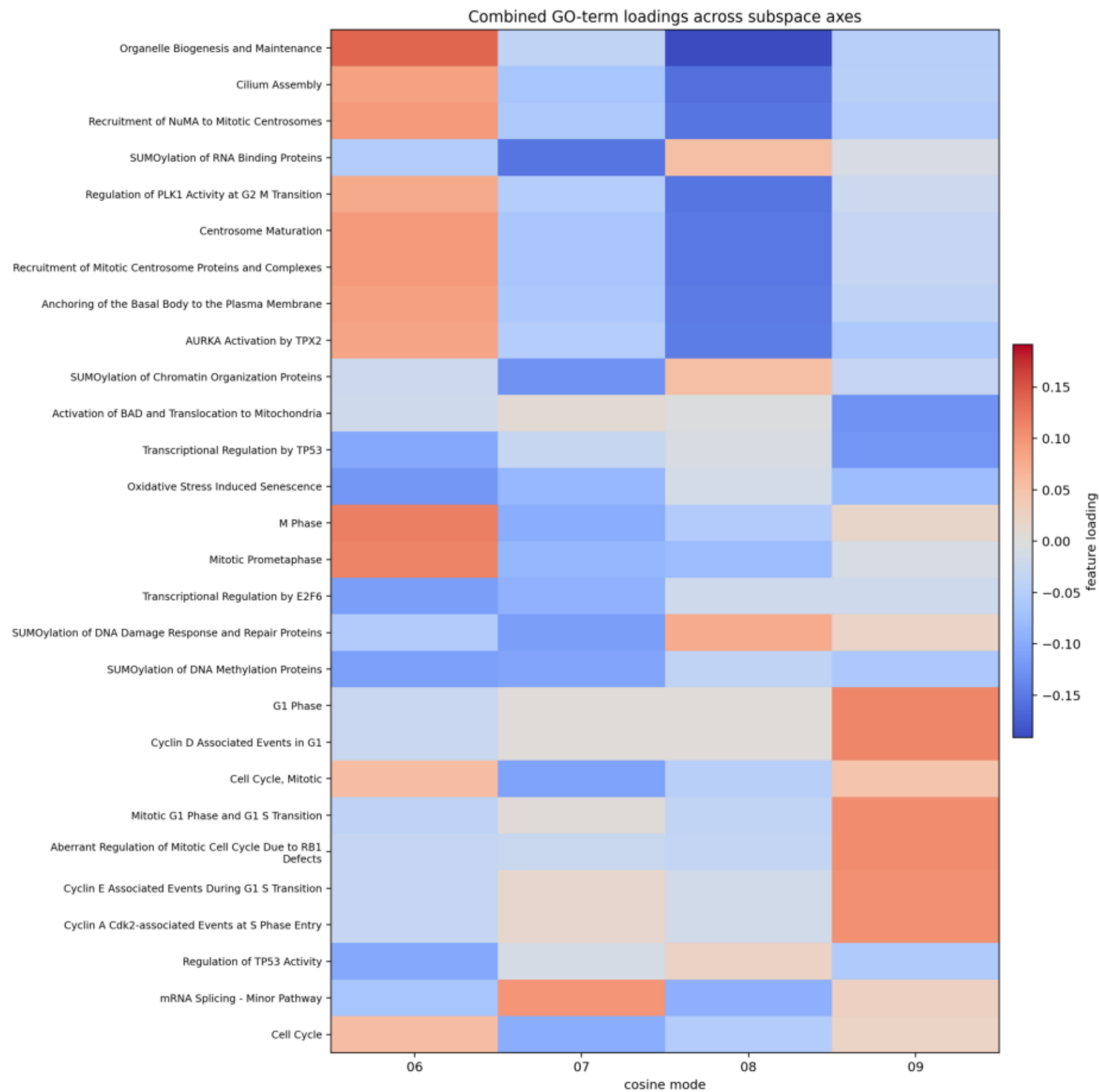
Rank 7: binary / adaptive_modes_06_09 Combined signed GO-term feature loadings across subspace eigenmodes
