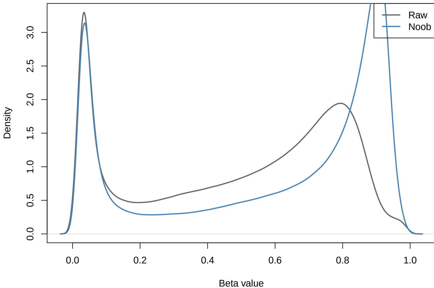
Raw versus Noob beta-value distributions
