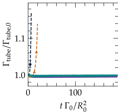
(a) Tube circulation
