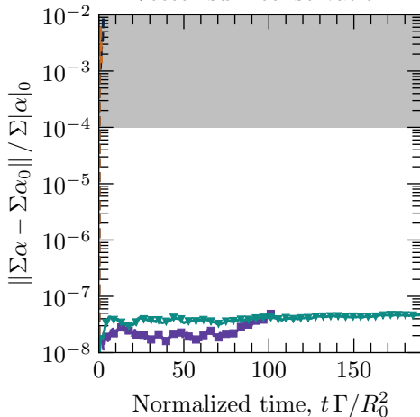
Vector-sum conservation
