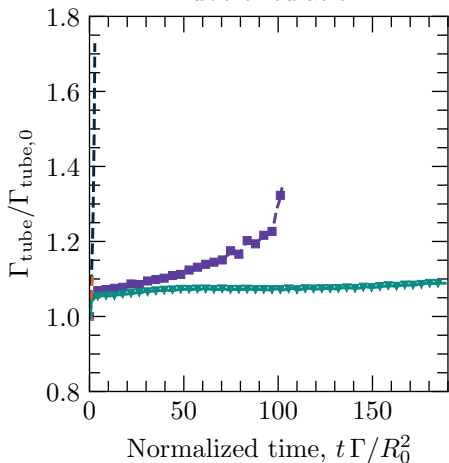
Tube circulation
