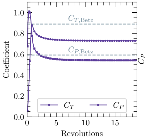
Rotor performance coefficients
