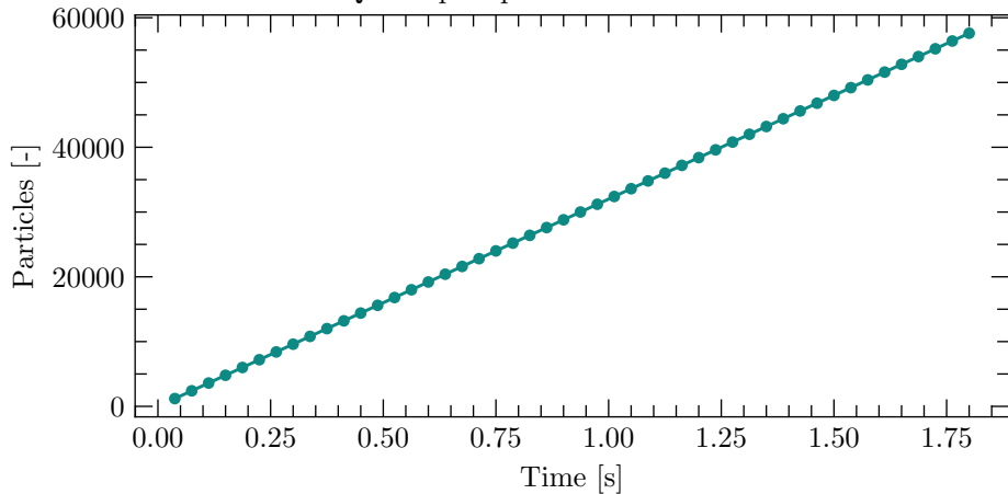
Quadcopter particle count evolution
