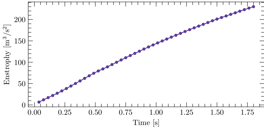
Quadcopter wake enstrophy history
