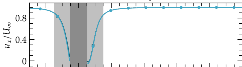
(a) Centreline, y/D = 0
