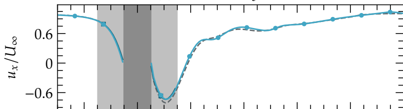
(a) Centreline, y/D = 0
