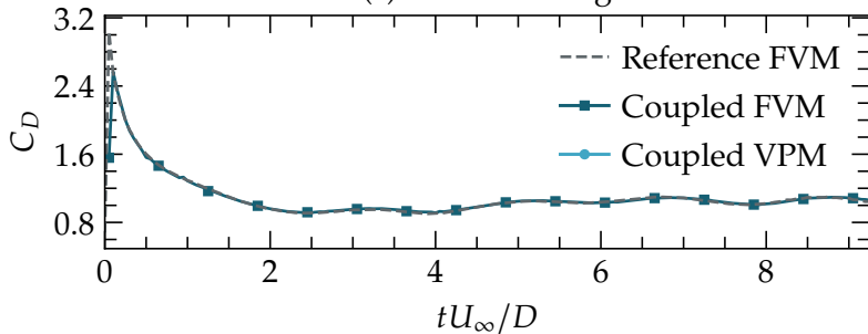
(c) Raw wall drag
