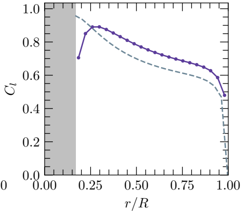
Sectional lift coefficient
