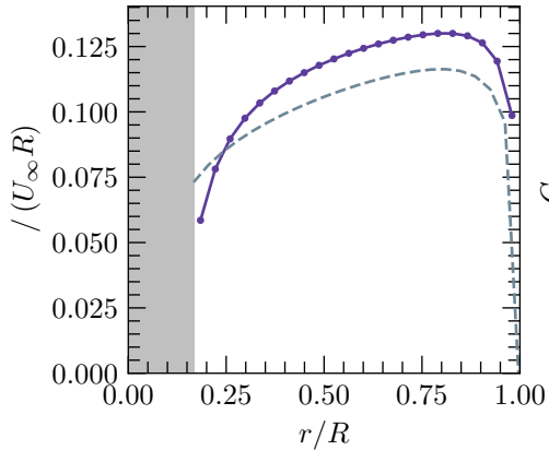
Normalized bound circulation
