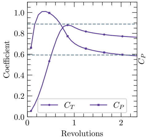
Rotor performance coefficients
