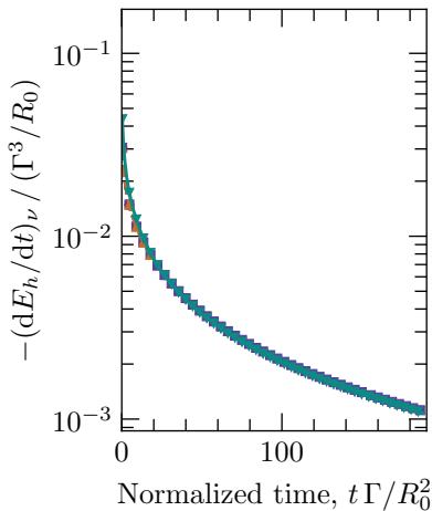
Modeled viscous dissipation
