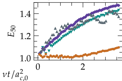
High-vorticity aspect
