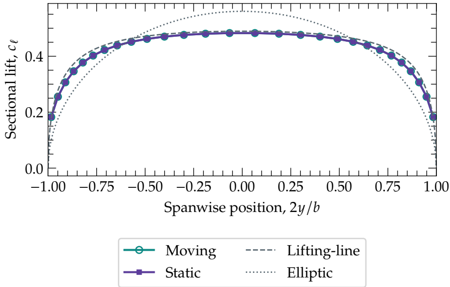
Spanwise c_\ell , \alpha = 5^\circ , AR=10
