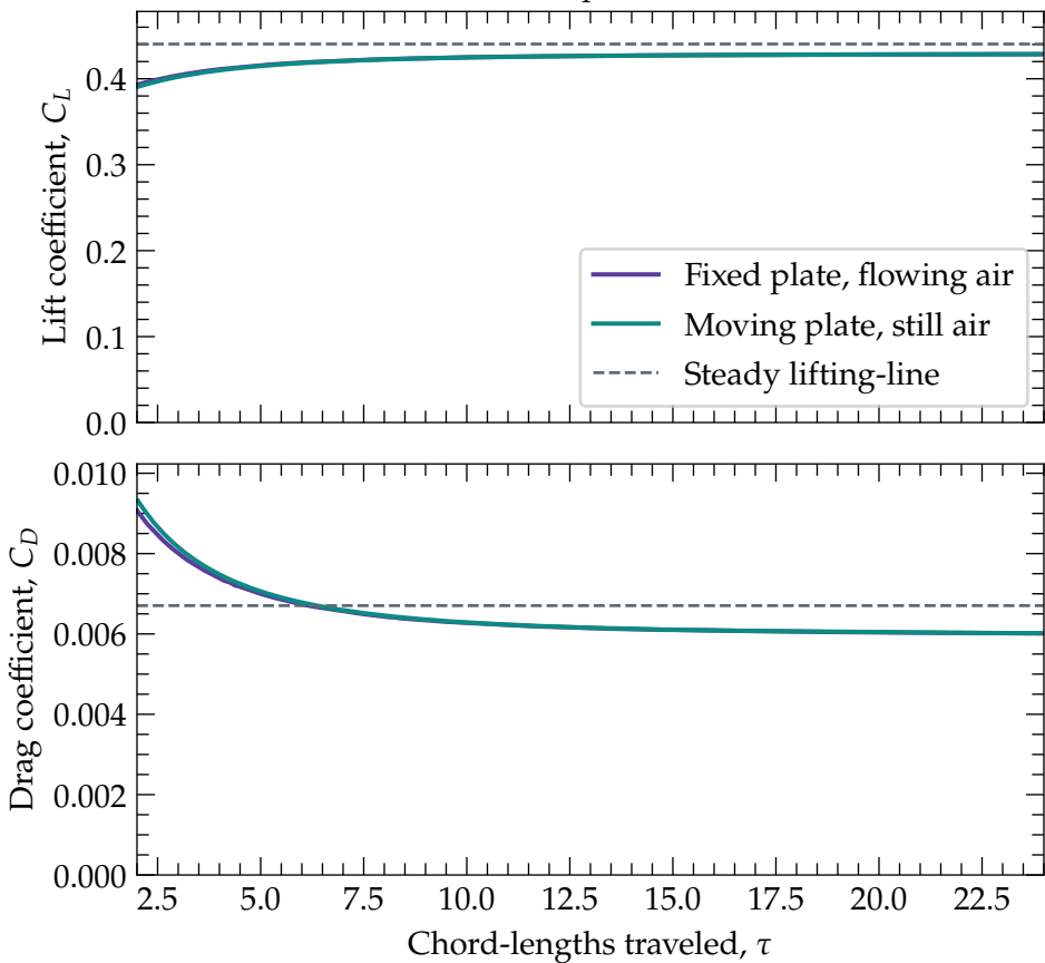
Wake development, \alpha = 5^\circ
