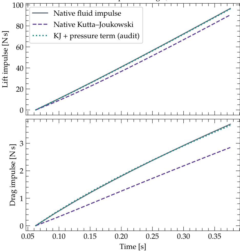
Audit: startup force budget, \alpha = 8^\circ
