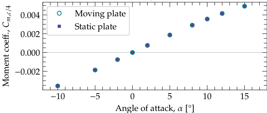
C_{m,c/4} vs \alpha
