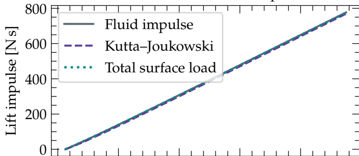
Surface force and fluid impulse
