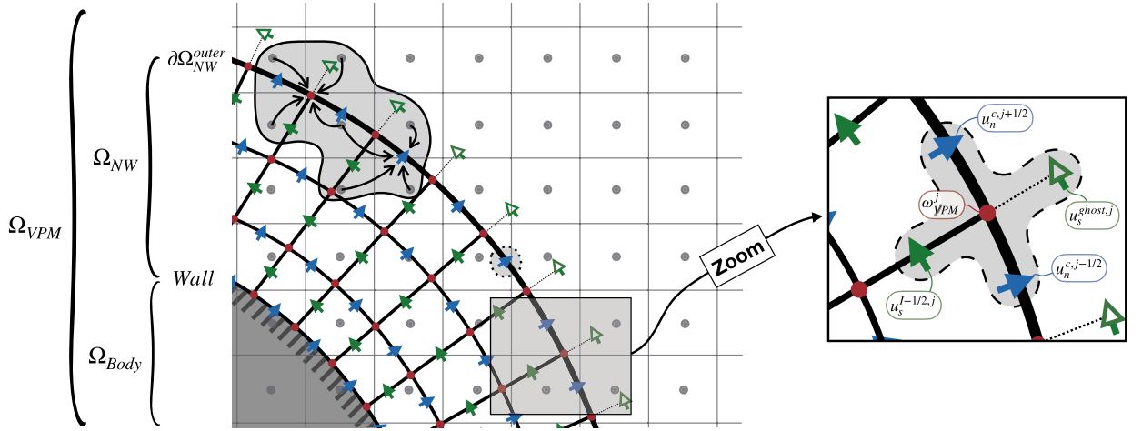
Fig. 3. Near-wall solver boundary condition enforcement: the NW solver staggered mesh is in the foreground with its variables u_s ( \rightarrow ), u_n ( \rightarrow ), \omega ( \bullet ) and u_s^{ghost} ( \rightarrow ); the VPM mesh ( \bullet ) is in the background. Spatial M2P M'_4 interpolation (step 1 - \rightarrow ). Correction of u_n to u_n^c (step 2.3 - \rightarrow ). Ghost tangential velocity computation (step 2.4 - \rightarrow - presented on the zoom). N.B: for the sake of clarity, the represented interpolation stencil is narrower than the one actually used; i.e., M'_4 (step 1).
