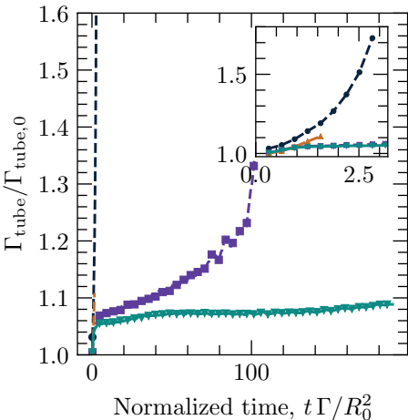
Tube circulation
