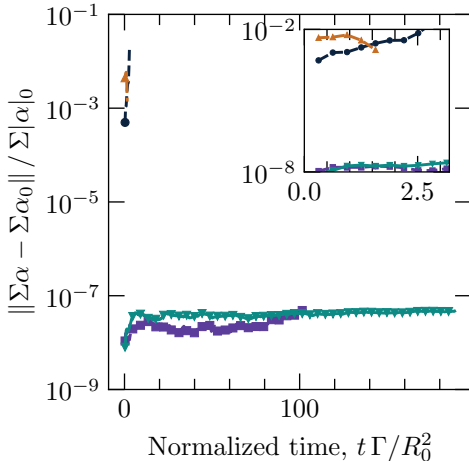
Vector-sum conservation
