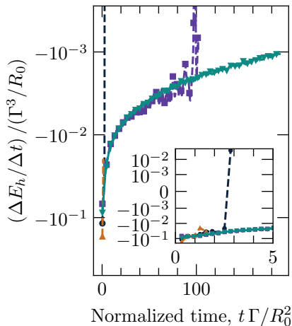
Resolved energy rate
