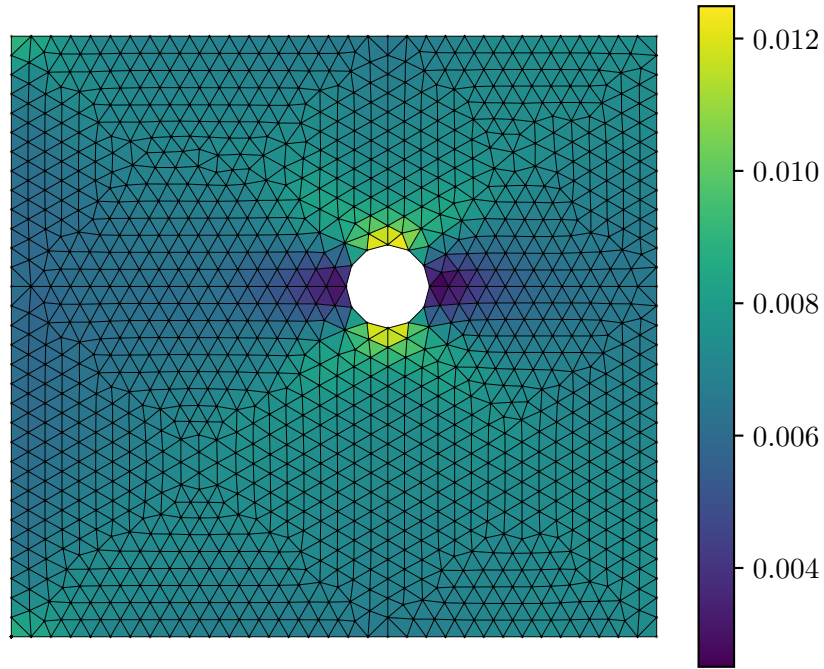
Predicted Strain \varepsilon_{xx}
