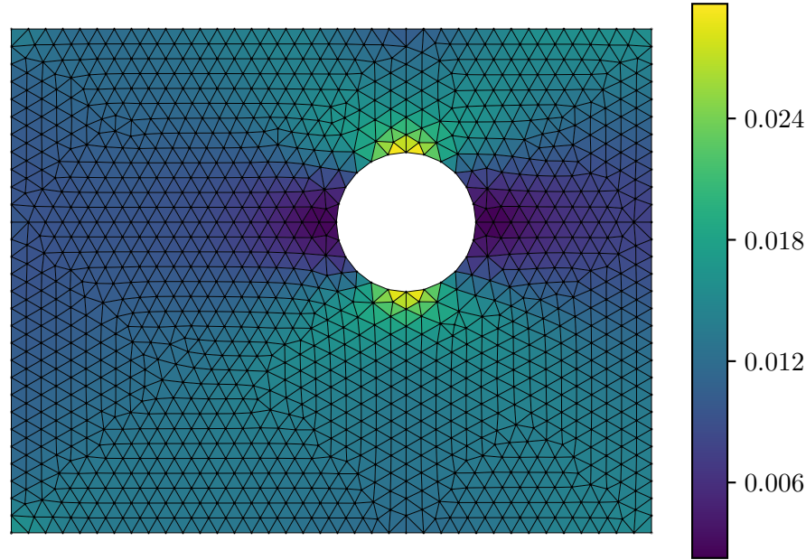
Predicted Strain \varepsilon_{xx}
