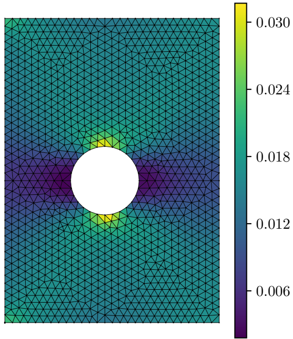
Predicted Strain \varepsilon_{xx}
