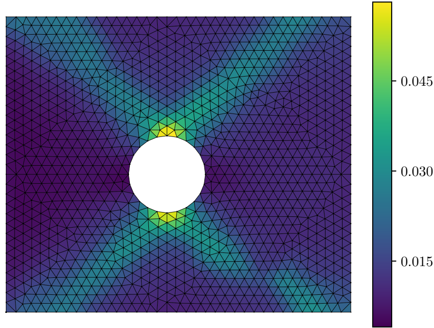
Predicted Strain \varepsilon_{xx}
