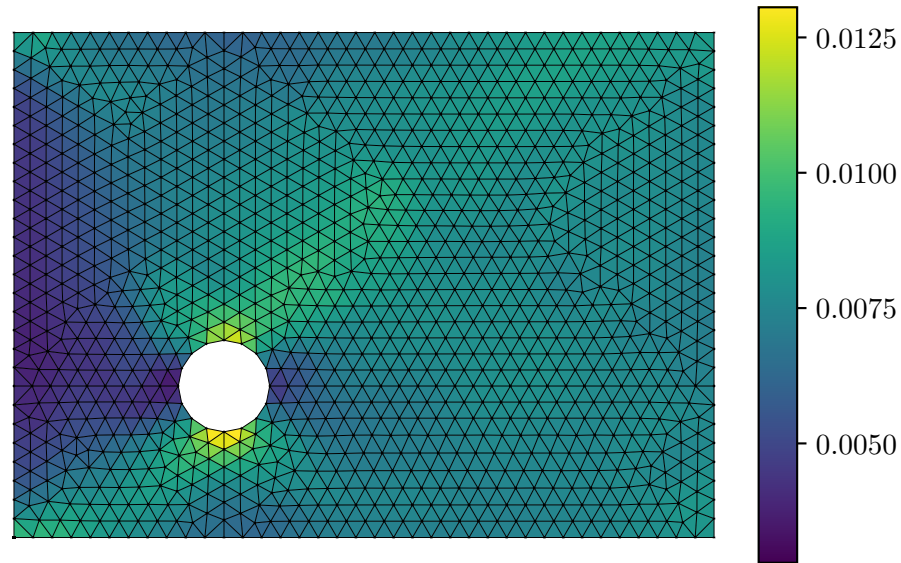
Predicted Strain \varepsilon_{xx}
