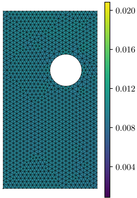
Predicted Strain \varepsilon_{xx}
