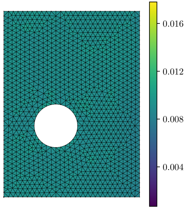
Predicted Strain \varepsilon_{xx}
