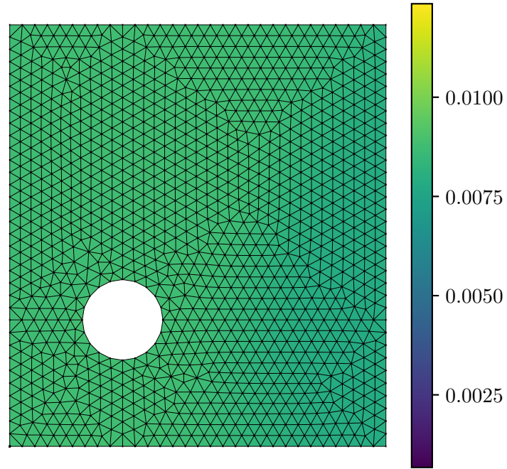
Predicted Strain \varepsilon_{xx}
