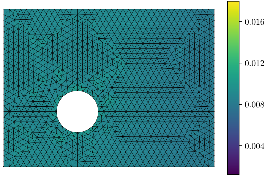
Predicted Strain \varepsilon_{xx}
