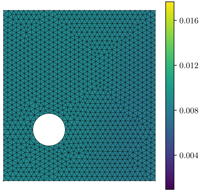
Predicted Strain \varepsilon_{xx}
