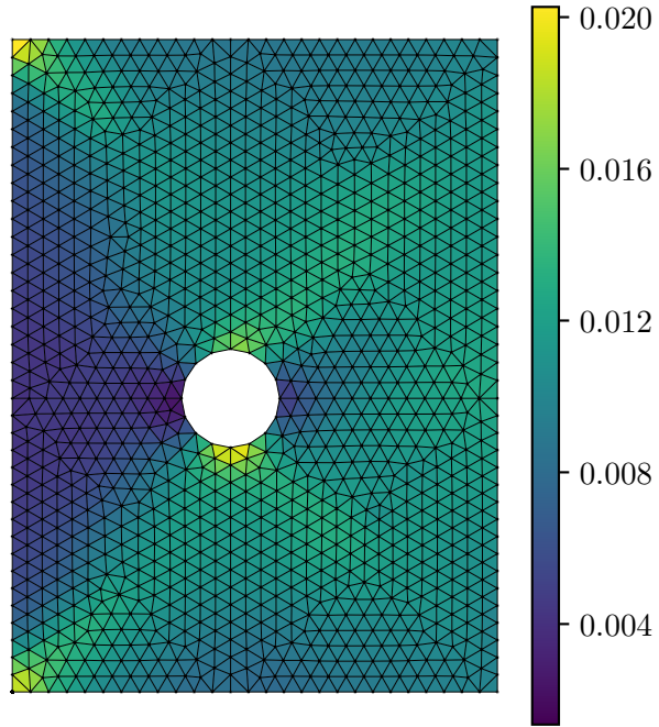
Predicted Strain \varepsilon_{xx}
