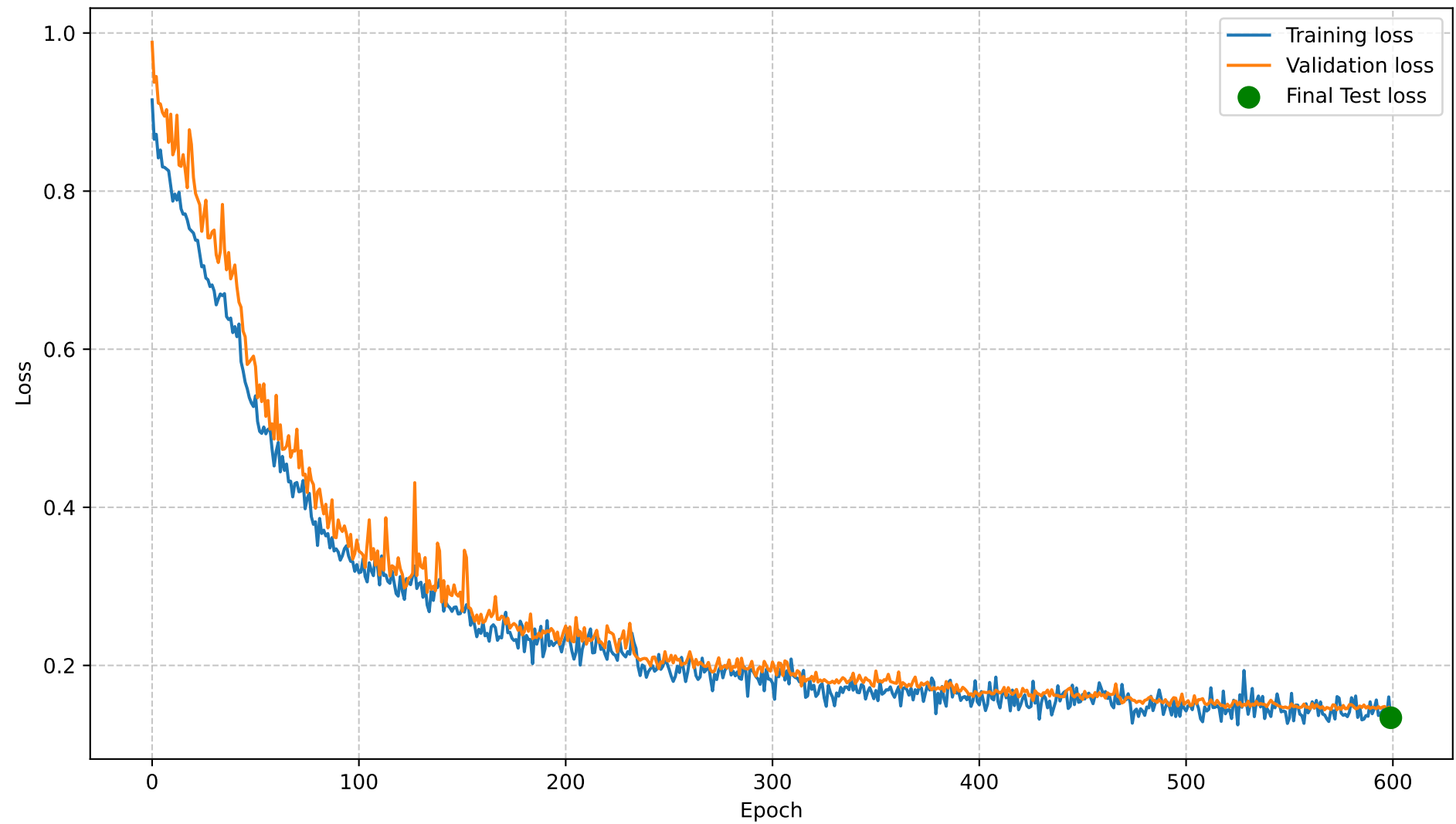
Losses Plot
